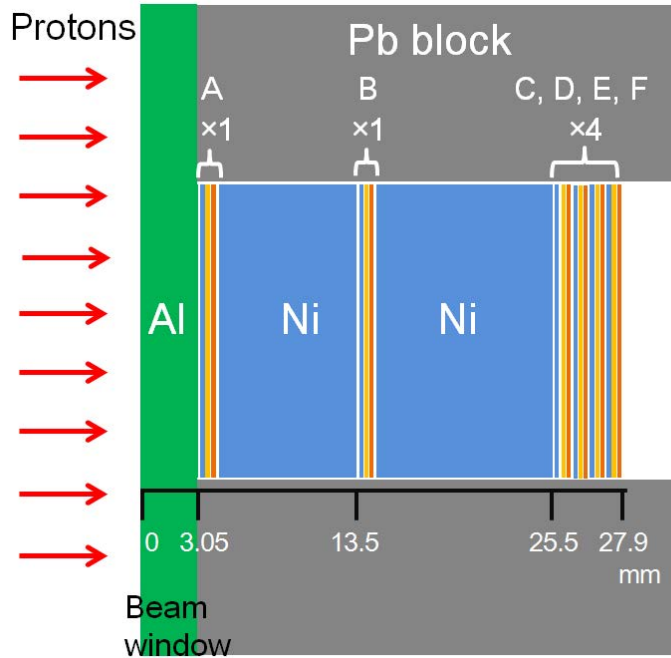
Fig. 2 Schematic illustration of six specimen positions (A-F) in a cavity of 3.2 mm in diameter, inside a Pb block of 40 \times 40 \times 38 \text{ mm}^3 for 150 MeV proton irradiation at room temperature. At each position, six specimens (two Ni, two Au, and two Cu discs) of 0.1 mm thickness and 3 mm diameter were inserted.
