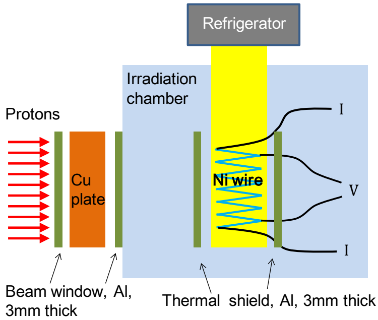
Figure 1 Schematic illustration of the setup used for the electrical resistance measurements. The electrical resistance of the Ni wire (0.1 mm in diameter) in the irradiation chamber was measured at 20 K during proton irradiation. A Cu plate was inserted between the two beam windows.
