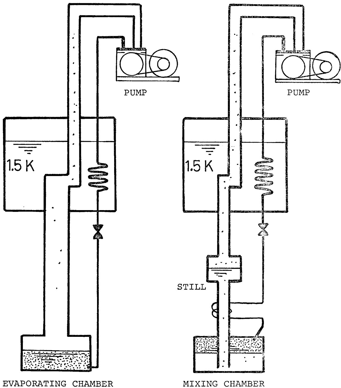
Figure 2.6 Schematic flow diagram of the \text{He}^3 evaporation refrigerator and \text{He}^3\text{-He}^4 dilution refrigerator.
