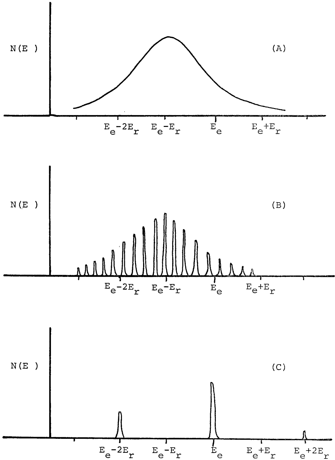
Figure 3.2 The gamma-rays emission spectra
