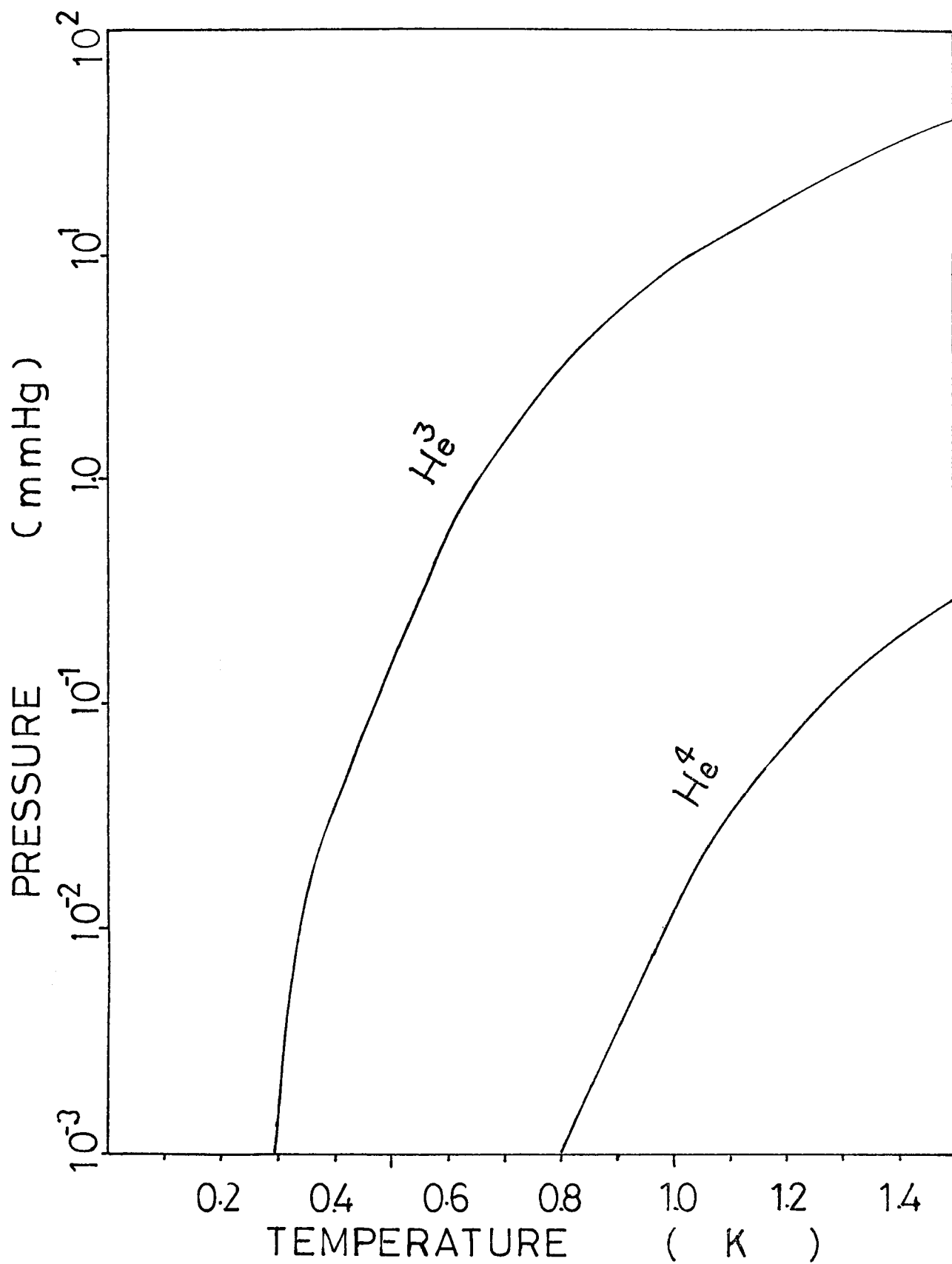
Figure 2.4 Saturated vapor pressure versus temperature for liquid helium-3 and liquid helium-4.
