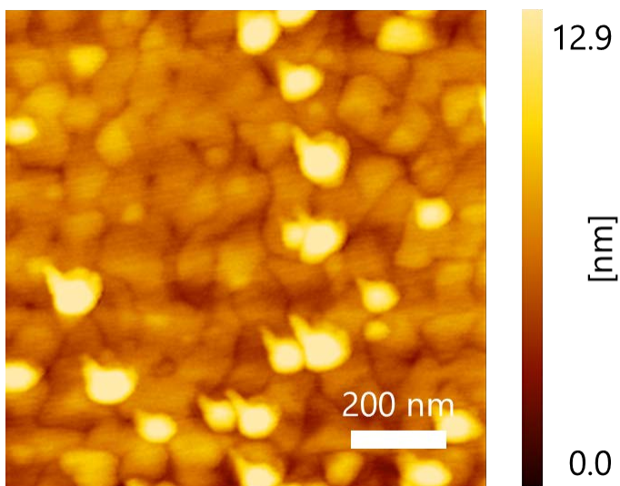
Figure 4. AFM image of \text{Ni}_{1-x}\text{Mg}_x\text{O} thin film obtained from source solution with a Mg concentration of 50%.
