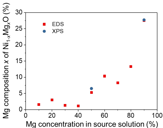
Figure 3. Dependence of the Mg composition of the \text{Ni}_{1-x}\text{Mg}_x\text{O} thin film on the Mg concentration in the precursor solution.
