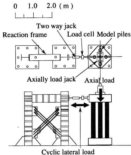
Fig.1 Test apparatus
