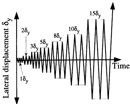
Fig.4 Applied load path
