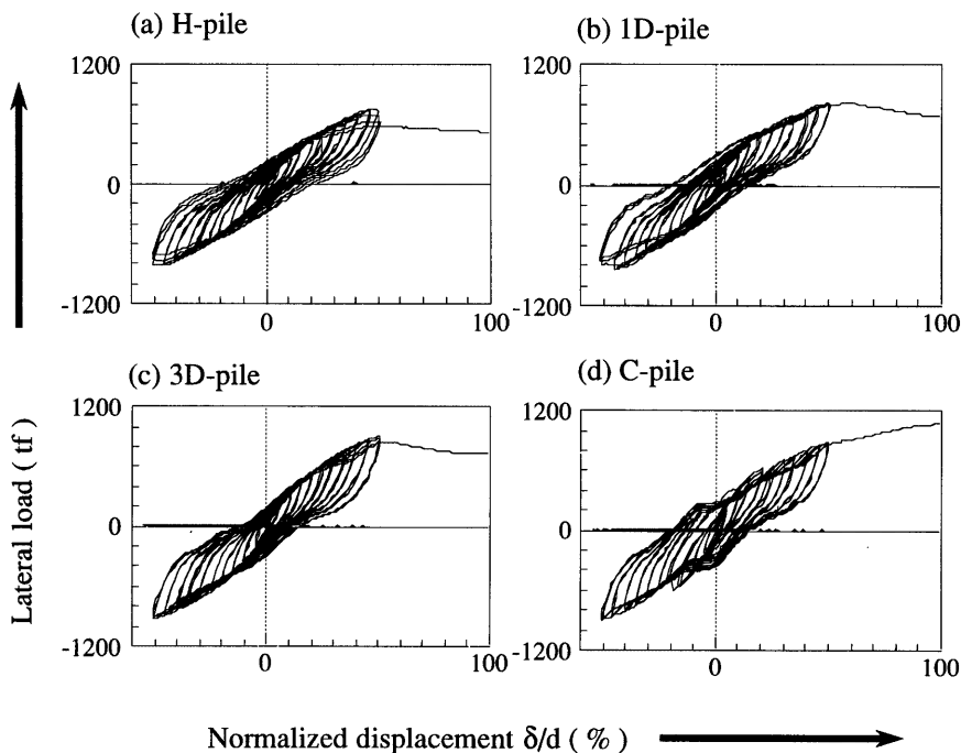
Fig.12 Load-displacement relations
