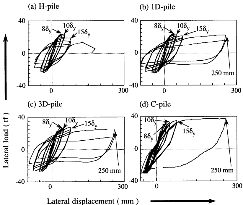
Fig.5 Load-displacement relation
