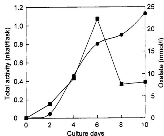
Fig. 1. Changes in the production of oxalate and the total glyoxylate dehydrogenase activity during the cultivation of Tyromyces palustris . Circles, oxalate production; squares, total enzyme activity.
