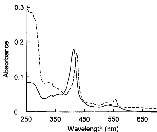
Fig. 2. UV and visible spectra of the heme fragment measured in the presence of glyoxylate and FMN fragment. —, Without supplement; ----, after the addition of glyoxylate and FMN fragment.
