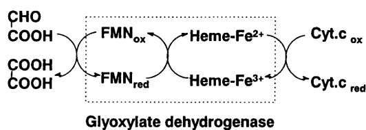
Fig. 3. A proposed scheme of electron-transferring function of the flavohemoprotein glyoxylate dehydrogenase during the dehydrogenation of glyoxylate to form oxalate in the presence of cytochrome c .
