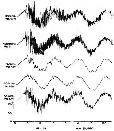
Fig. 3a. Sea level (along the Pacific Coast).
