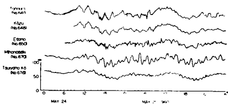
Fig. 3f Sea level (along the Japan Sea Coast).
