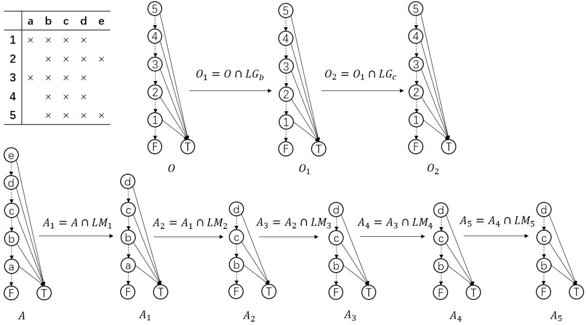
Fig. 2.2 The process for computing O^{(1)} and O^{(1)(2)} where O = \{b, c\} on a sample dyadic context represented with a cross table on the upper-left using the Z-TCA algorithm. The results of O^{(1)} and O^{(1)(2)} are O_2 and A_5 , correspondingly.
