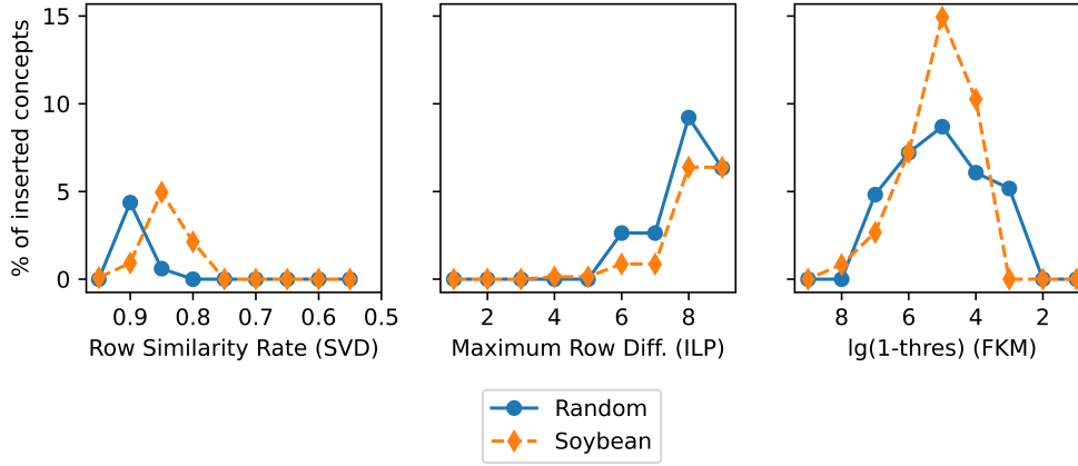
Fig. 3.8 The percentage of inserted concepts in the reduced concept lattice of different methods applying the OR rule in Experiment 1.
