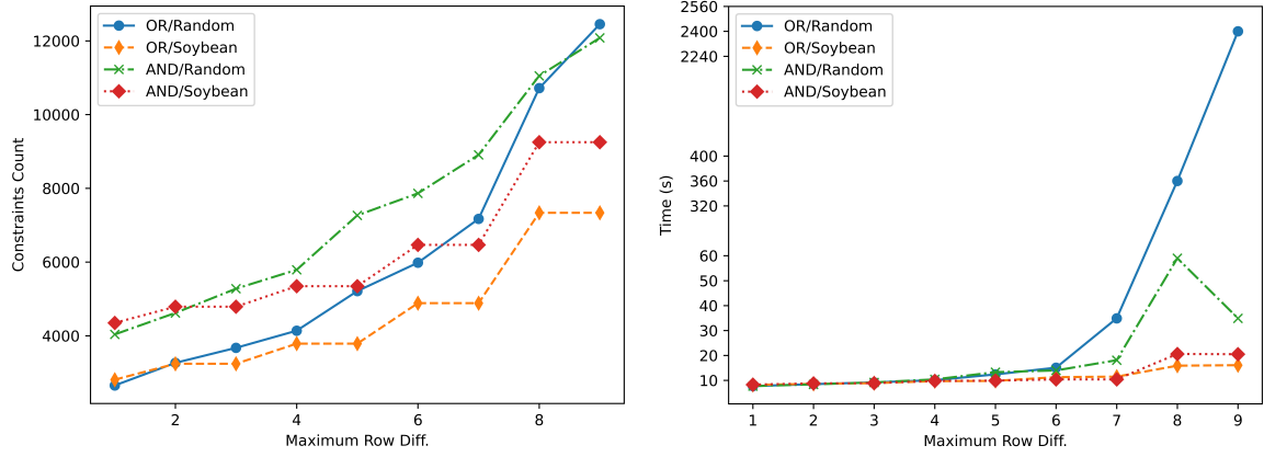
Fig. 3.9 The run time and the number of variables of our method in Experiment 1.
