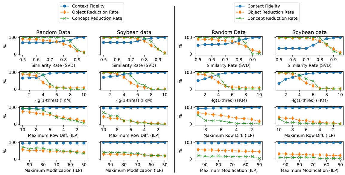
Fig. 3.7 Left: Statistics of the three methods on two datasets applying the OR rule. Right: Statistics of these methods on the same datasets applying the AND rule. For the SVD method, the rank of the reconstructed matrix is set to 3/4 . For the FKM method, the m value is set to 1.05. \lg(\cdot) in the captions of the second row means \log_{10}(\cdot) . For our model, \varepsilon_r is set to 6 for the test cases shown in the fourth row, and the \varepsilon_m is set to infinite for the cases shown in the third row.
