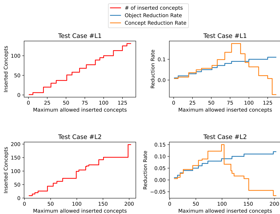
Fig. 3.11 The reduction rates and number of inserted concepts of our method on the two large test cases applying the OR rule, with different settings for the maximum allowed inserted concepts.
