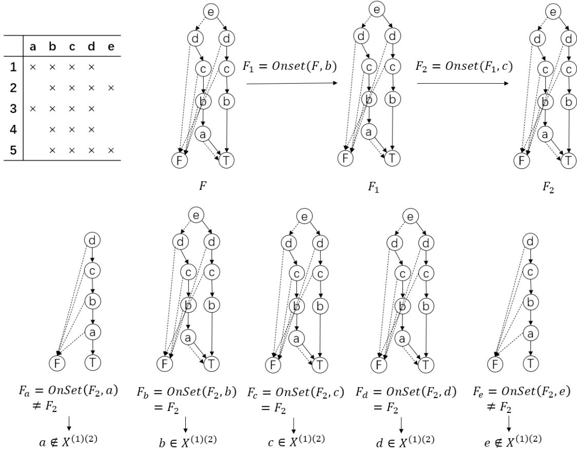
Fig. 2.4 The process for computing X^{(1)(2)} where X = \{b, c\} on a sample dyadic context represented with a cross table on the upper-left using the ZDD-PropriIm algorithm.
