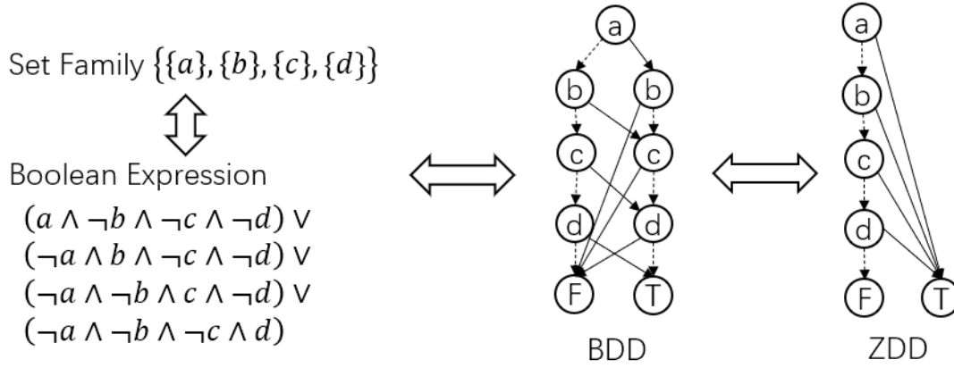
Fig. 2.1 An example of a set family and its equivalent Boolean expression, its BDD representation, and ZDD representation. In the BDD and ZDD representation, the label on each node represents its corresponding variable; the edges in solid lines are the HI edges, and the edges in dashed lines are the LO edge; the node labeled T and F represent the TRUE node, and the FALSE node, respectively.
