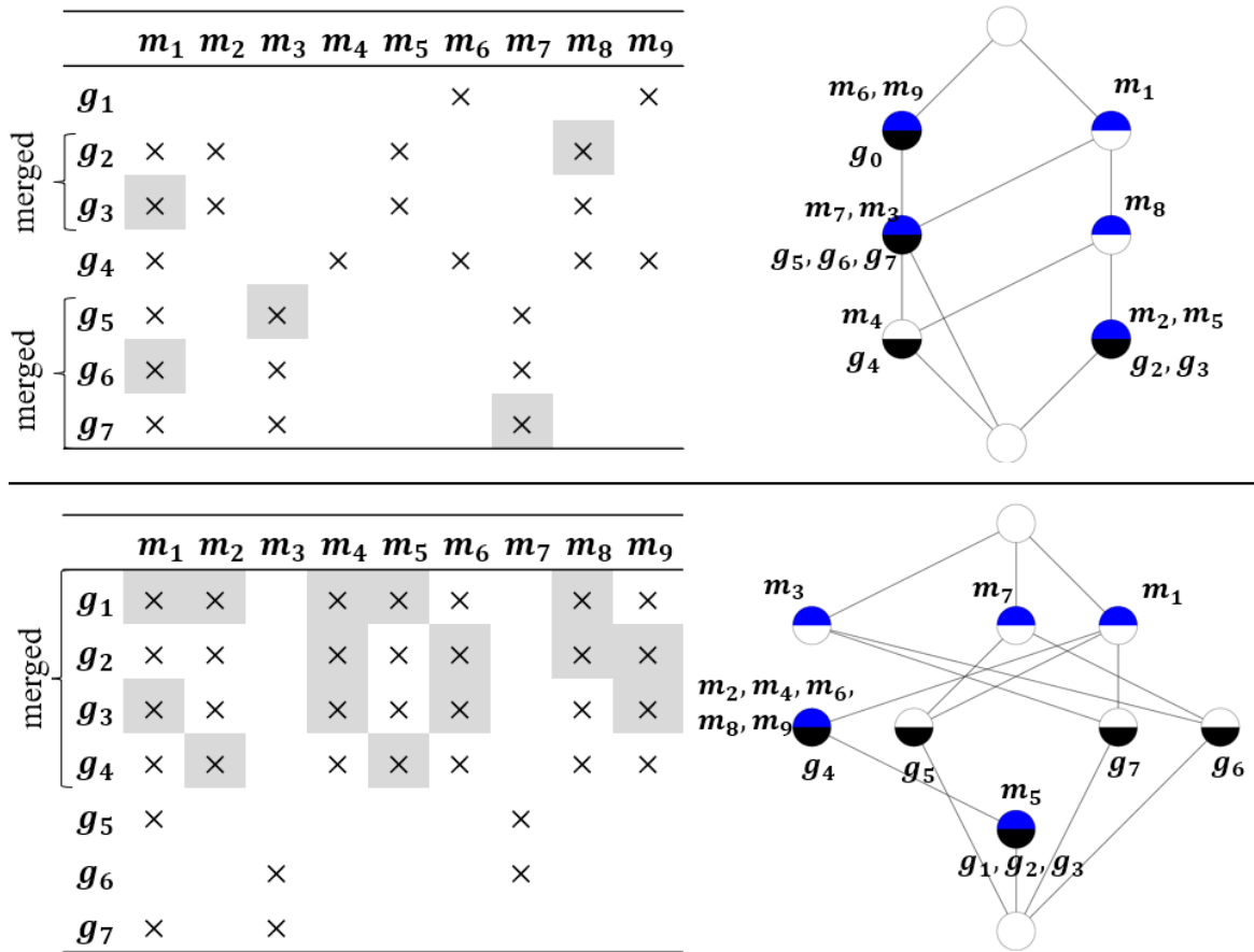
Fig. 3.4 Upper row: a sample reduction plan for the context shown in the left panel of Fig. 3.3. Lower row: the reduction plan given by the method proposed in [17]. Shaded cells represent the modified incidences.
