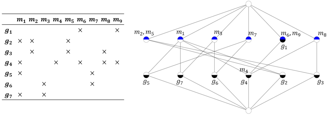
Fig. 3.3 Left: A sample context. Right: The concept lattice corresponding to the context in the left panel.
