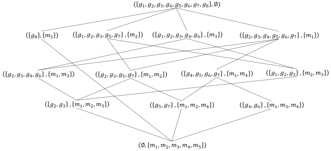
Fig. 1.3 The fully annotated diagram of the concept lattice corresponding to the context in the left panel of Fig. 1.2.
