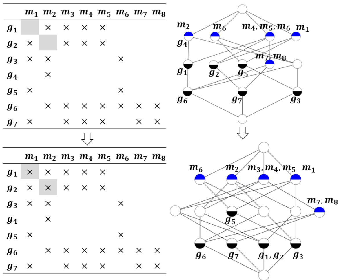
Fig. 3.5 Upper row: a sample context and its corresponding concept lattice. Lower row: the reduced context after merging object g_1 and g_2 with the OR rule, with its corresponding concept lattice shown on the right.
