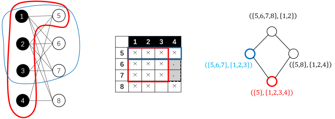
Fig. 4.4 An sample pair of overlapping bi-cliques and their structure hole. Left: A bipartite network with two overlapping maximal bi-cliques framed out in red and blue, separately. Middle: The bi-adjacent matrix of the network on the left. The aforementioned maximal bi-cliques correspond to the red and blue rectangles, separately. The gray cells filled with dots represent their structure hole. Right: the concept lattice representing all maximal bi-cliques from the network. The aforementioned bi-cliques correspond to the concepts marked out in blue and red, separately.
