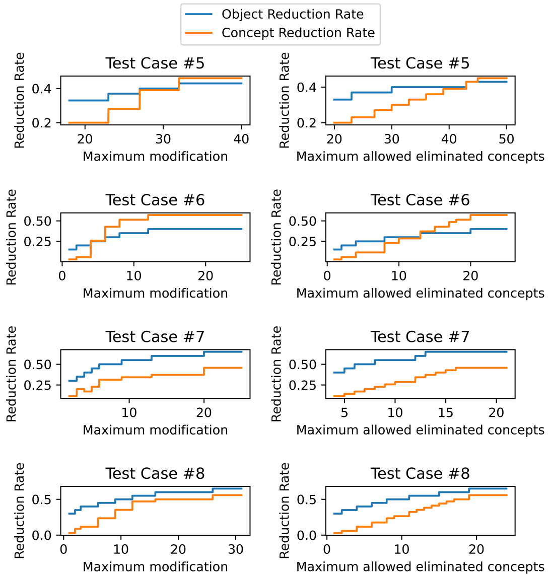
Fig. 3.12 The reduction rates of our method on the four small test cases applying the AND rule, with different settings for the maximum allowable modifications and maximum allowed eliminated concepts. Note that the concept reduction rate equals the percentage of eliminated concepts.
