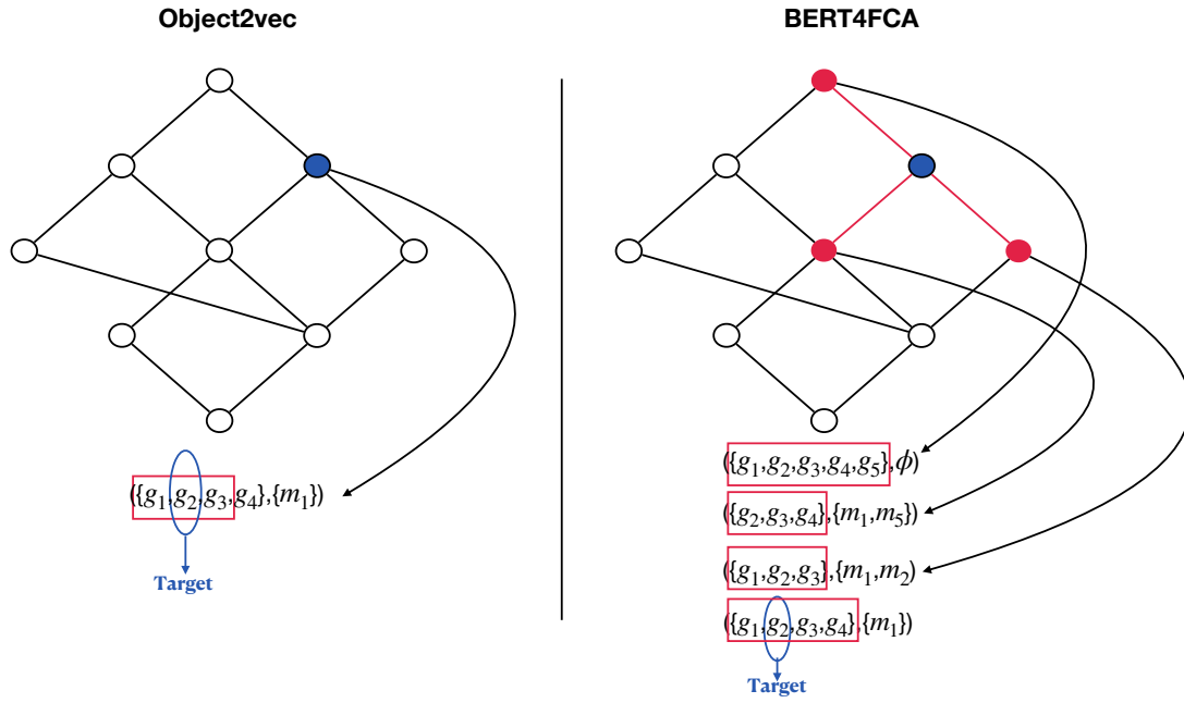
Fig. 5.3 The comparison of how much information from a concept lattice is learned and used when predicting an object by two methods, with object2vec shown on the left and BERT4FCA shown on the right. The target object to be predicted is circled in blue. The information used for predicting the object is shown in red.
