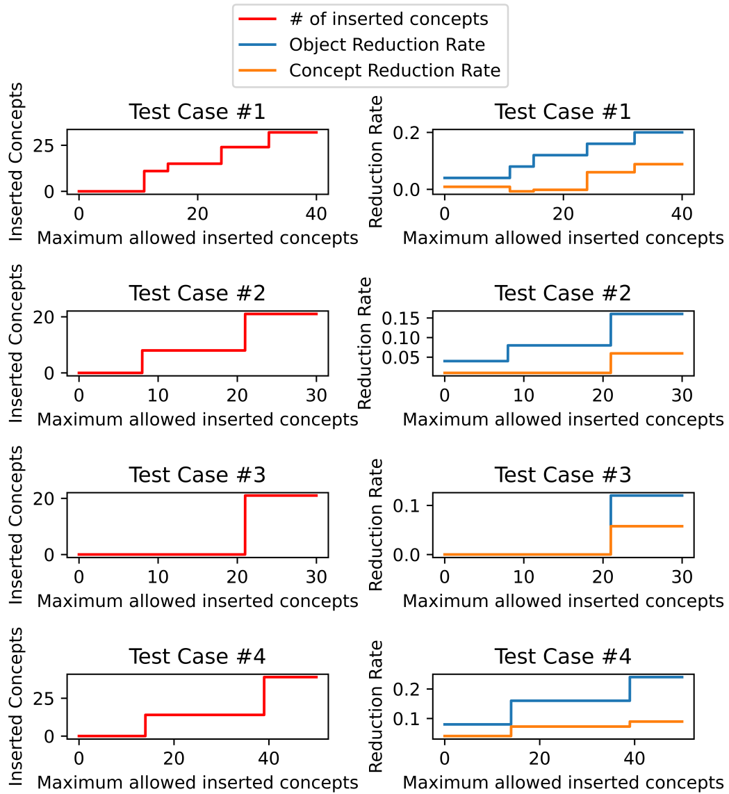
Fig. 3.10 The reduction rates and number of inserted concepts of our method on the four small test cases applying the OR rule, with different settings for the maximum allowed inserted concepts.
