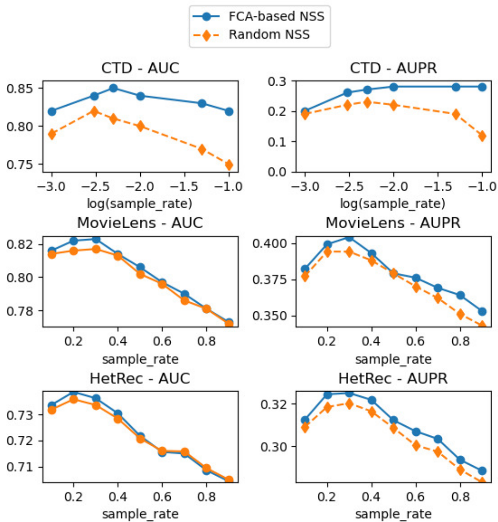
Fig. 4.7 The AUC and AUPR scores with different sample rates.
