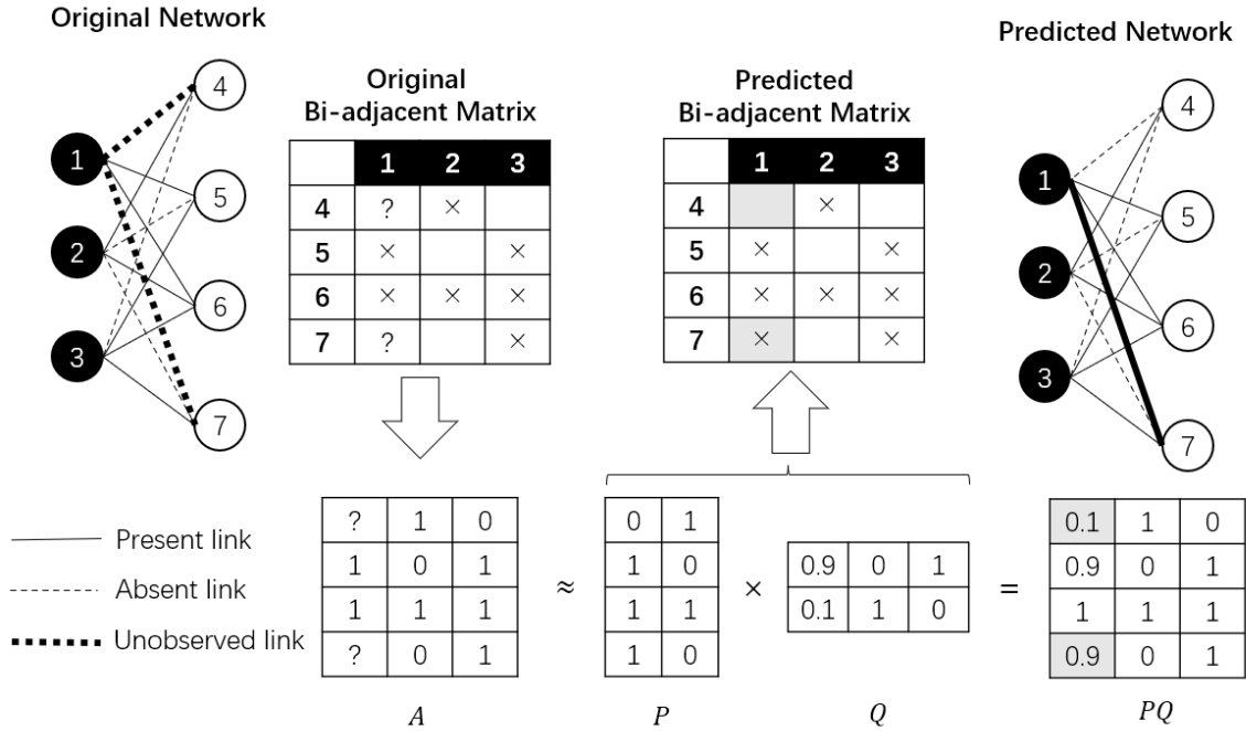
Fig. 4.1 An example of the working flow of the MF-based bipartite link prediction. In the bi-adjacent matrices, present links, absent links, and unobserved links are represented with crosses, empty cells, and question marks, correspondingly. The bi-adjacent matrix of the original network is converted into a numerical matrix A , which is then decomposed into the product of P and Q . In the reconstructed matrix PQ , the confidence values of two node pairs with unobserved links (v_1, v_4) and (v_1, v_7) are 0.1 and 0.9 separately, so finally, we only predict a new link between (v_1, v_7) .
