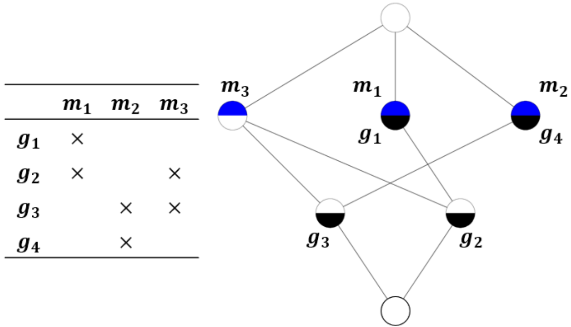
Fig. A.2 Left: The sample context to be reduced in Example 2. Right: The corresponding concept lattice of the context on the left.
