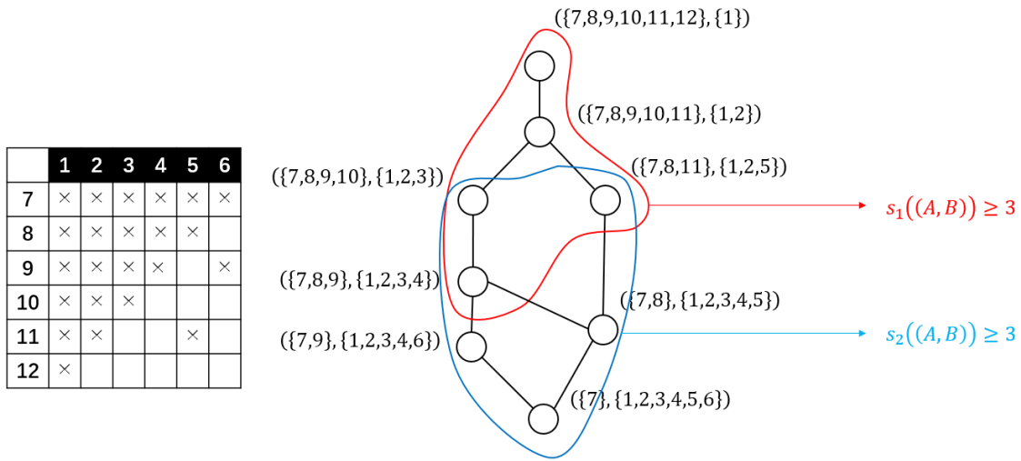
Fig. 4.5 An example of the iceberg-shaped sections of the concept lattice corresponding to the bi-cliques with component sizes exceeds a threshold 3.
