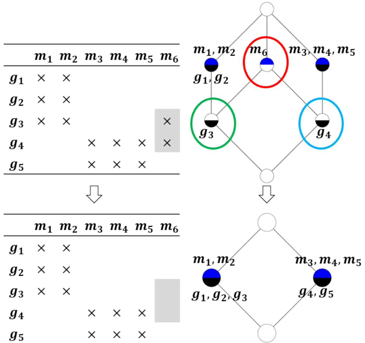
Fig. 3.6 Upper row: a sample context and its corresponding concept lattice. Lower row: the reduced context after merging g_3 with g_1 and g_2 , and merging g_4 with g_5 applying the AND rule, with its corresponding concept lattice shown on the right.
