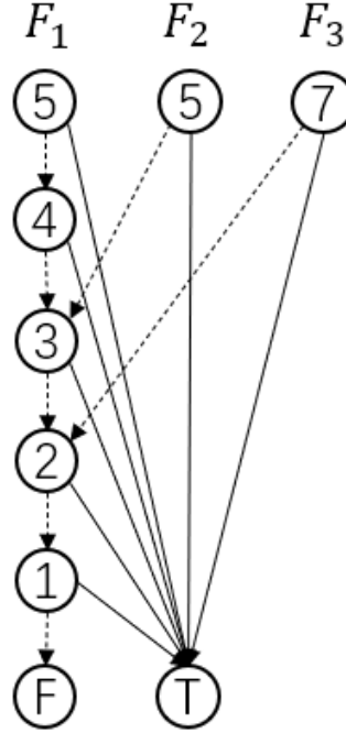
Fig. 2.3 An example of the node usage of three ZDDs: F_1 = \{\{1\}, \{2\}, \{3\}, \{4\}, \{5\}\} , F_2 = \{\{1\}, \{2\}, \{3\}, \{5\}\} , F_3 = \{\{1\}, \{2\}, \{7\}\} .
