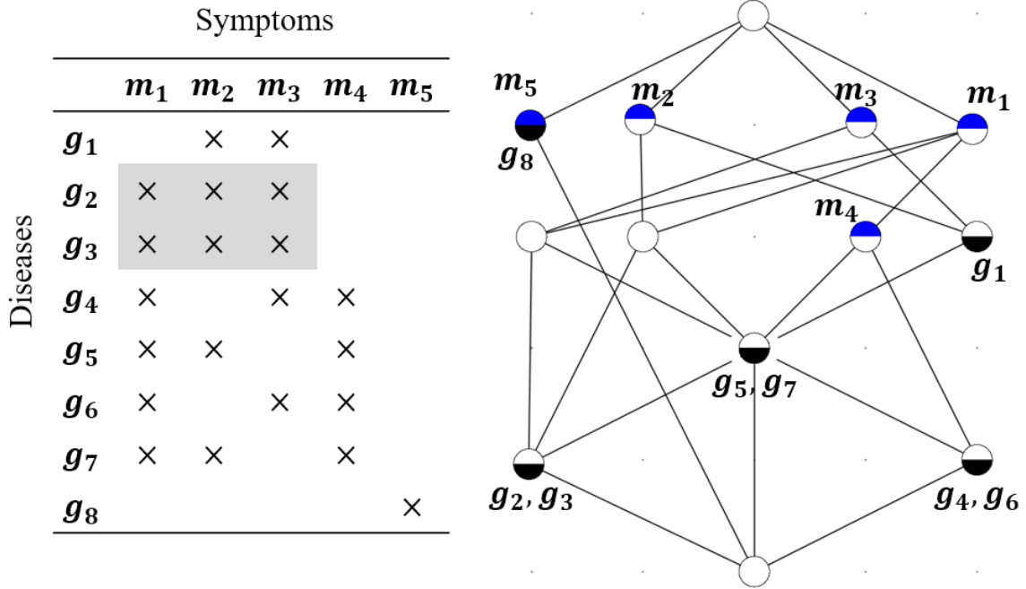
Fig. 1.2 Left: A sample formal context of symptoms of some diseases in an abstract form. Right: The concept lattice corresponding to the context in the left panel. The concept lattice is shown in the form of a line diagram. Please refer to Section 1.2 for how to read the diagram. The fully annotated form of the diagram is shown in Fig. 1.3.
