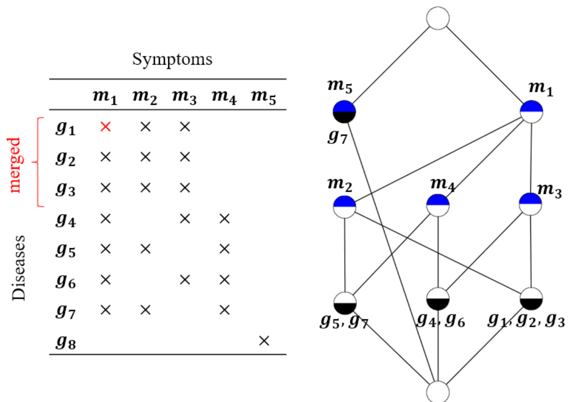
Fig. 3.1 Left: The reduced formal context after merging Diseases g_1, g_2 and g_3 in the context shown in left panel of Fig. 1.2. Right: the corresponding concept lattice of the reduced context.
