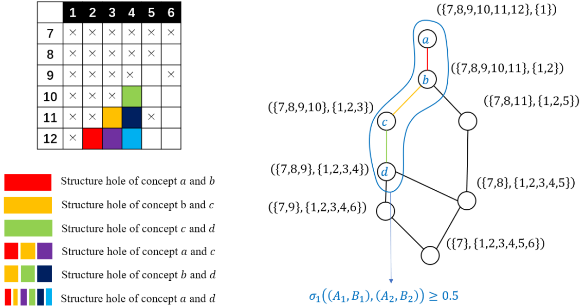
Fig. 4.6 An example of a chain-shaped cluster corresponding to a group of non-trivial overlapping bi-cliques. The structure hole of each pair of concepts is marked with cells in different colors. It is clear that the structure hole of the maximum and minimum concept, i.e. , concept a and d contains that of any other pair of concepts from the group.
