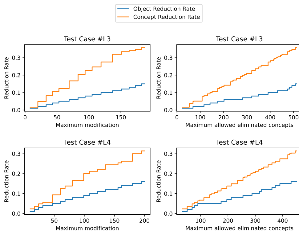
Fig. 3.13 The reduction rates of our method on the two large test cases applying the AND rule, with different settings for the maximum allowable modifications and maximum allowed eliminated concepts. Note that the concept reduction rate equals the percentage of eliminated concepts.
