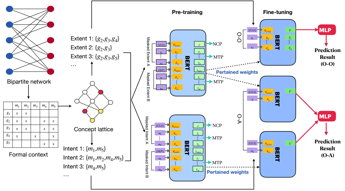
Fig. 5.2 An overview of the working flow of our method.
