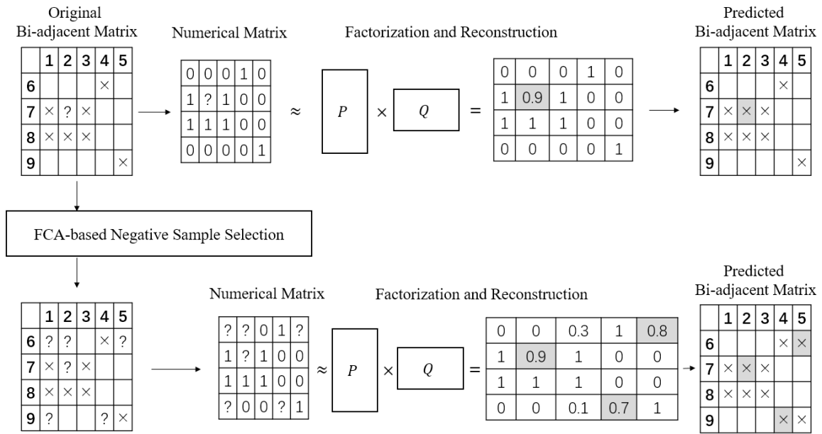
Fig. 4.2 The comparison of the working flow of the raw MF method and our joint method. The upper row depicts the working flow of the raw MF method, while the lower row depicts that of our method.
