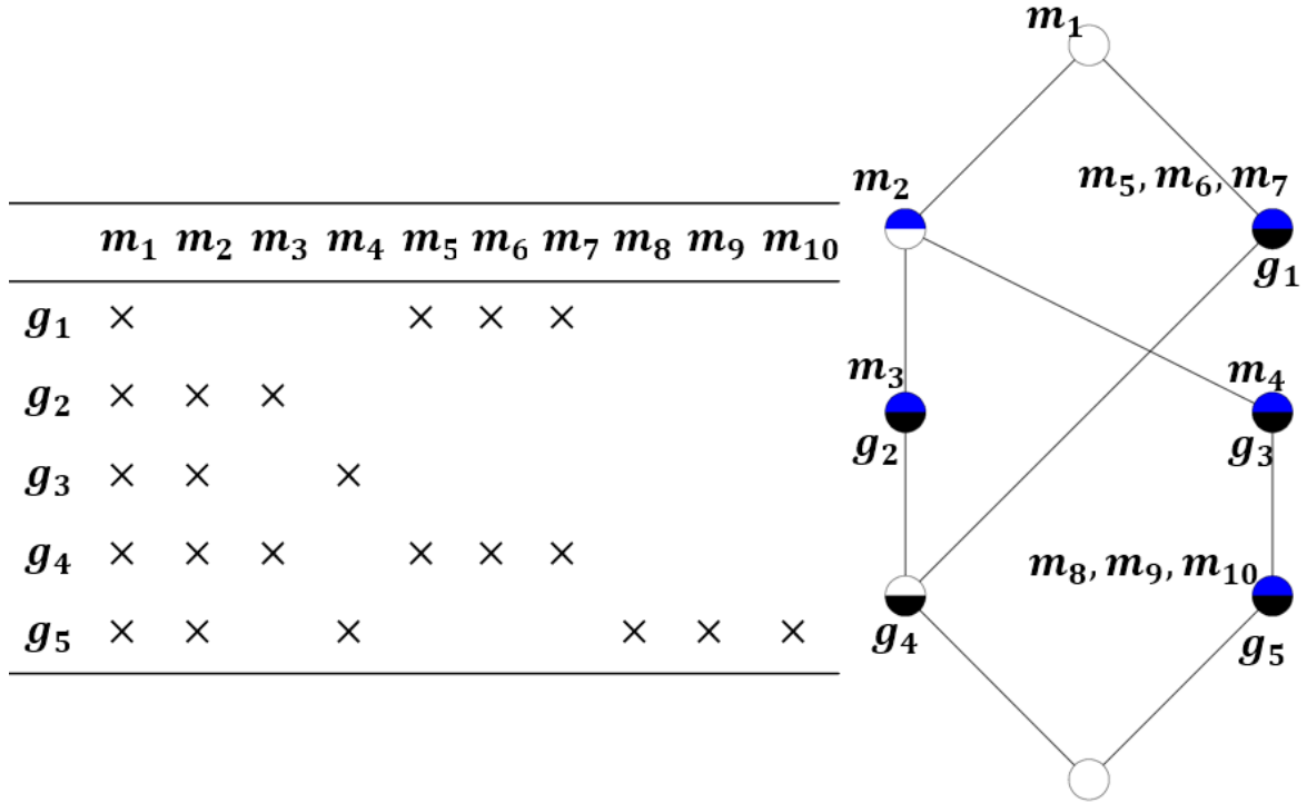
Fig. A.1 Left: The sample context to be reduced in Example 1. Right: The corresponding concept lattice of the context on the left.
