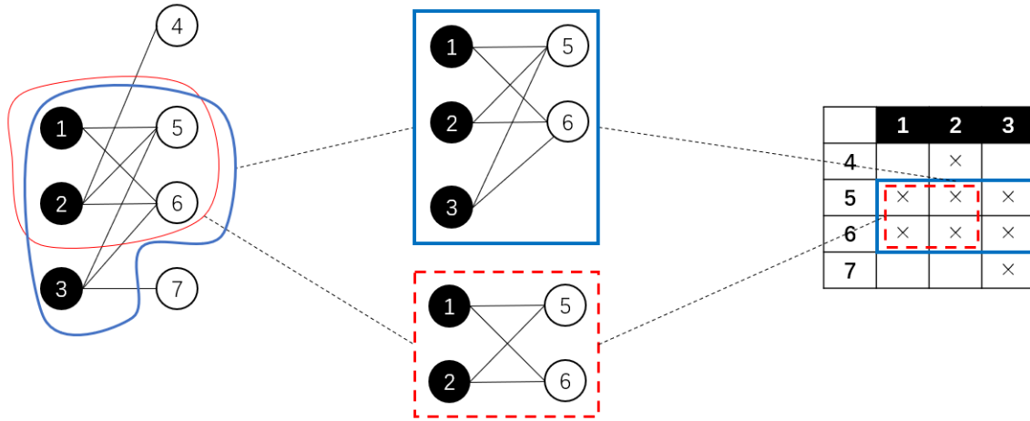
Fig. 4.3 An example of a bi-clique and a maximal bi-clique. The sub-network framed out in red from the bipartite network on the left is a bi-clique, which corresponds to the rectangle framed with red dash lines in the bi-adjacent matrix shown on the right. However, it is not a maximal bi-clique because it is a sub-network of another bi-clique framed in blue. The latter bi-clique is a maximal bi-clique, for it corresponds to the rectangle framed with solid blue lines on the right, which is a maximal rectangle box filled with crosses with rows and columns permutable.
