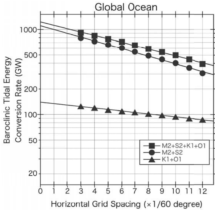
Fig. 3. The globally integrated baroclinic tidal energy conversion rates for the semidiurnal (solid circles) and diurnal tidal constituents (solid triangles) and the sum of the four major tidal constituents (solid squares) obtained using various horizontal grid spacing of 1/20^{\circ} – 1/5^{\circ} . Superposed on each plot is the least squares fitting line.
