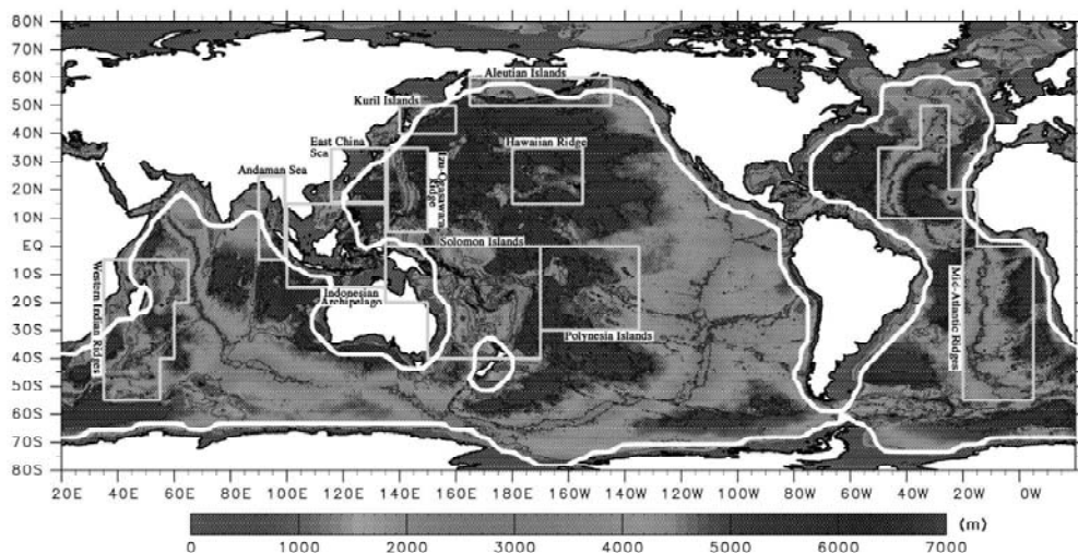
Fig. 1. The whole model domain and the bathymetry. The regions including the prominent topographic features are indicated by straight lined squares. The thick white line indicates the boundary between the open ocean and the coastal and marginal seas.
