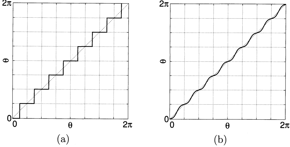
Figure 1: Multilevel functions which are the essences of the complex-valued activation functions: (a) Multilevel sigum function with K = 8 . (b) Multilevel sigmoid function with K = 8 and \epsilon = 0.1 .
