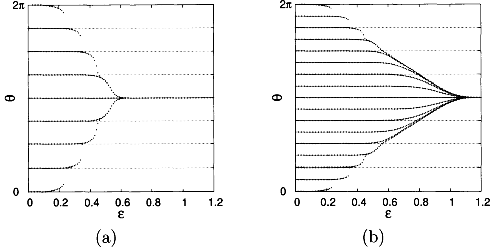
Figure 3: Bifurcation of the CSIGM function for the variation of the nonlinearity parameter \epsilon . (a) K = 8 . (b) K = 16 .
