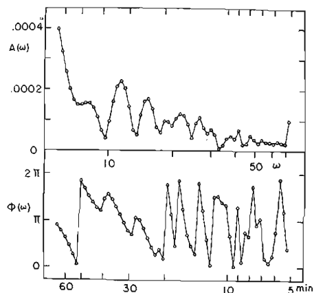
Fig. 20. Amplitude and phase spectra of the E-W component tilt at Amagase calculated from the data from June 9, 20:56 to 23:40, 1968.
