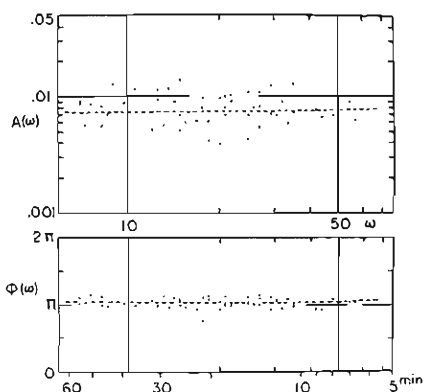
Fig. 11. Amplitude ratio and phase difference of the E-W component tilt at Oura to the atmospheric pressure. Unit of the ordinate of the ratio is second of arc/m.b.
