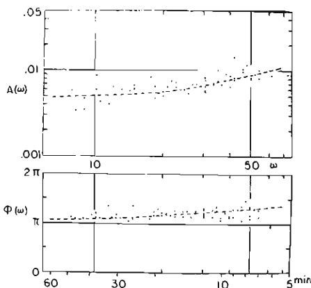
Fig. 15. Amplitude ratio and phase difference of the E-W component tilt at Akibasan to the atmospheric pressure. Unit of the ordinate of the ratio is second of arc/mb.
