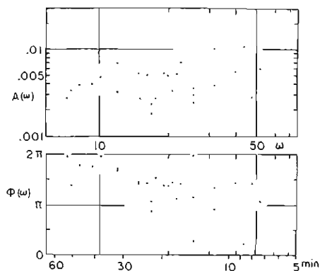
Fig. 22. Amplitude ratio and phase difference of the E-W component tilt at Amagase to the atmospheric pressure. Unit of the ordinate of the ratio is second of arc/mb.
