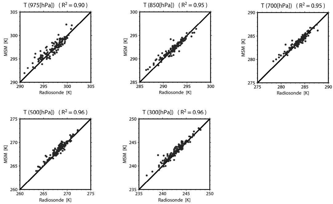
Fig. 8 The temperatures at the 975-hPa, 850-hPa, 700-hPa, 500-hPa, and 300-hPa levels from the radiosonde observations at the Tateno site (horizontal axis) and the mesoscale analyses at the corresponding grid (vertical axis).
