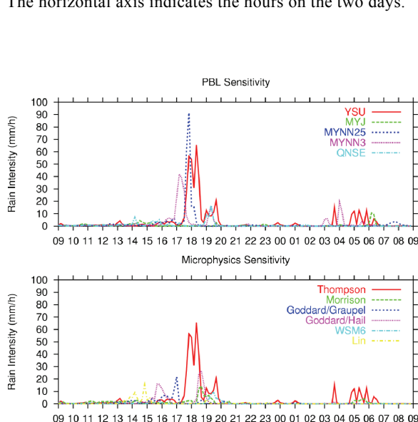
Fig. 3 The same as Fig. 2, except for those obtained by the PBL sensitivity experiments (upper panel) and the microphysics sensitivity experiments (lower panel).
