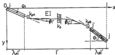
Fig. 4 Representation of member force and deformation.
