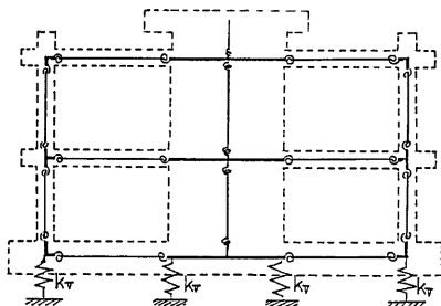
Fig. 3 Analytical model.
