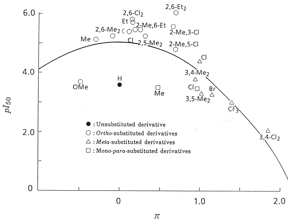
Fig. 2-2 Relationship of pI_{50} of 1- N -phenethyl compounds with the \pi value of anilide substituents.
