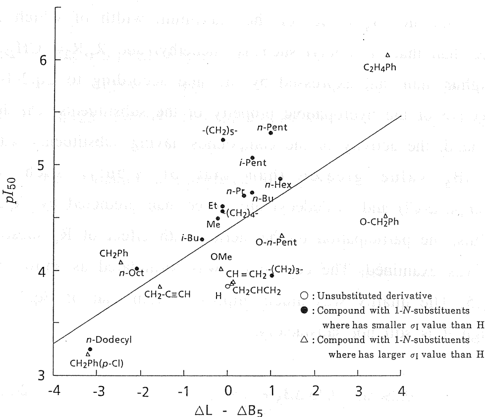
Fig. 2-7 Relationship of pI_{50} of 3-(2',6'-diethylanilide) compounds with the \Delta L and \Delta B_5 parameters for 1- N -Substituents.
