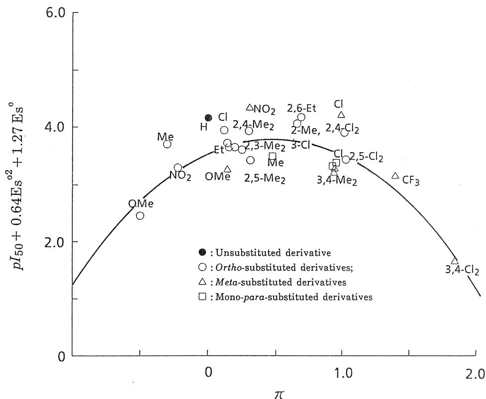
Fig. 2-5 Relationship of pI_{50} of 1- N -butyl compounds with the \pi and E_s^{\circ} parameters for anilide substituents.
