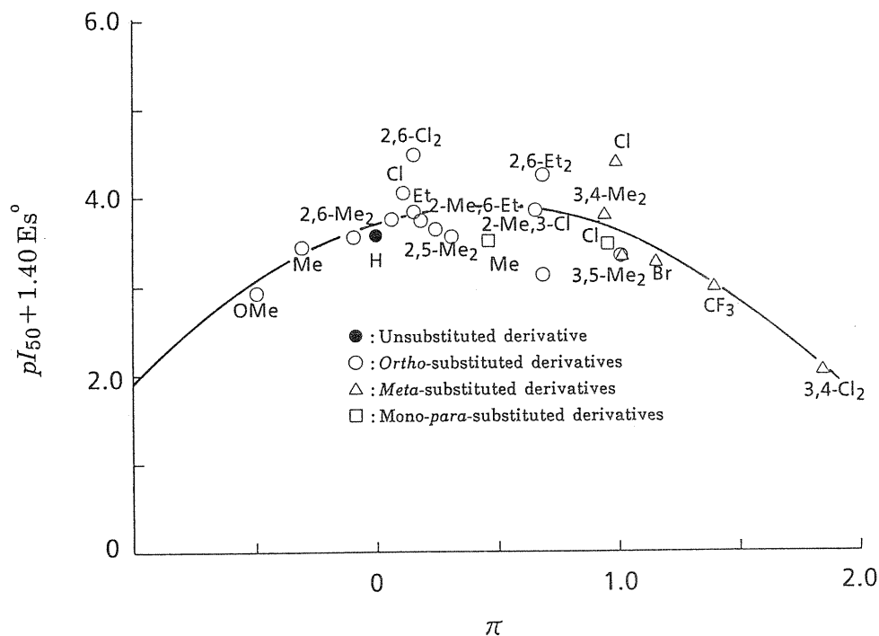
Fig. 2-3 Relationship of pI_{50} of 1- N -phenethyl compounds with the \pi and E_s^o parameters for anilide substituents.
