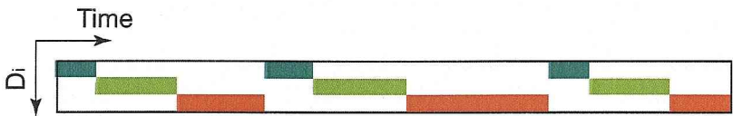
(a) Generated interval sequence of three dynamical systems
