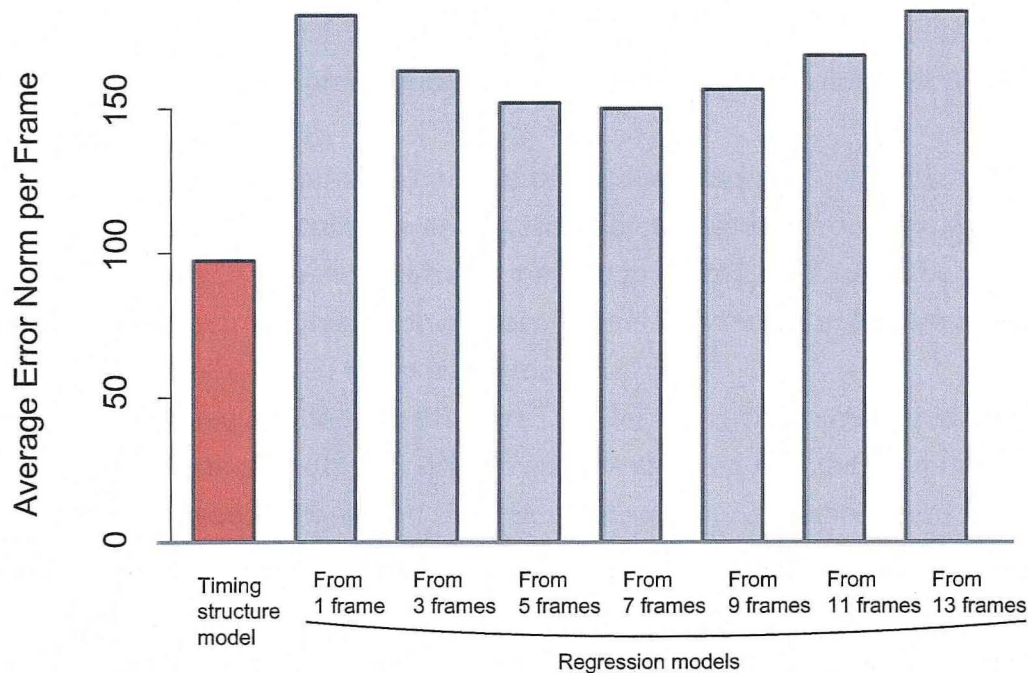
(b) Average error norm (per frame).
