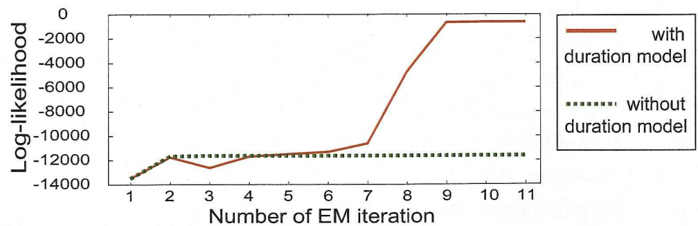
(b) The change of the overall log likelihood during the EM iteration
