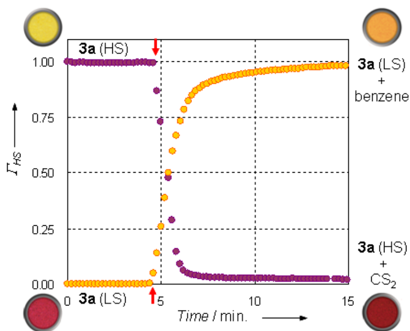
Fig. 9. Time dependence of the HS fraction of 3a under a benzene (yellow) and \text{CS}_2 (purple) atmosphere at 293 K. Red arrows indicate the starting points of guest injection (valve opening). The color circles are photos of samples.
