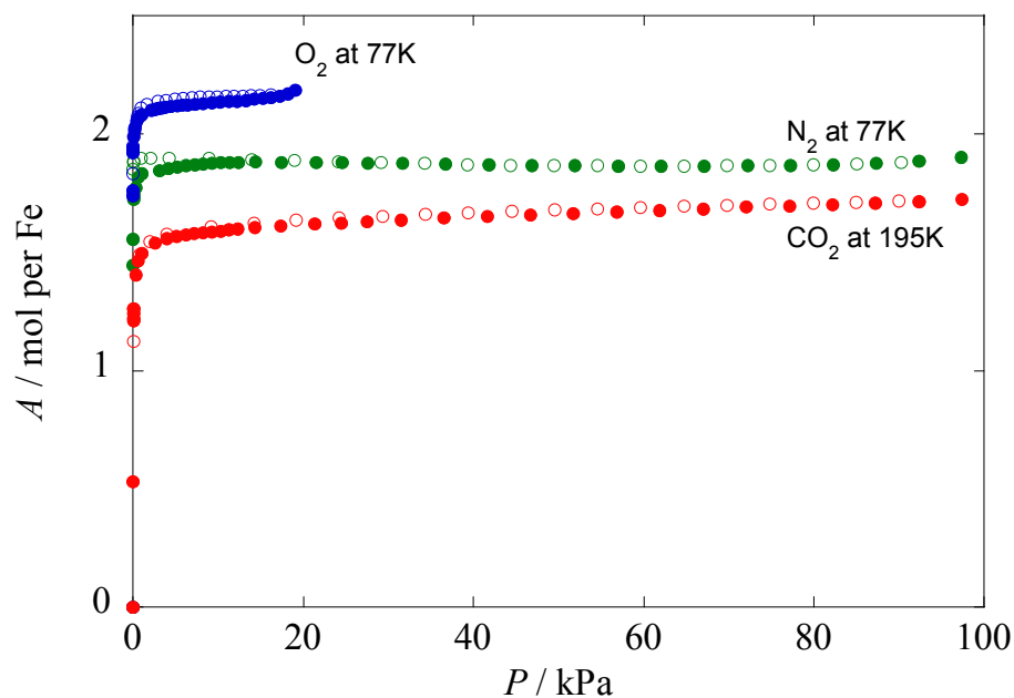
Fig. 3. Sorption and desorption isotherms for gases: (A) CO 2 in 1-LS (black), CO 2 in 1-HS (red), N 2 in 1-LS (green) and O 2 in 1-LS (blue) at 298 K in the pressure range from 10^{-6} to 100 kPa and equilibrium time of 120 sec., and (B) CO 2 , N 2 and O 2 in 1-LS (at low temperature): CO 2 (red), N 2 (green), O 2 (blue) in the pressure range from 10^{-6} to 100 kPa and equilibrium time of 120 sec. Filled and open circles express adsorption and desorption processes, respectively.
