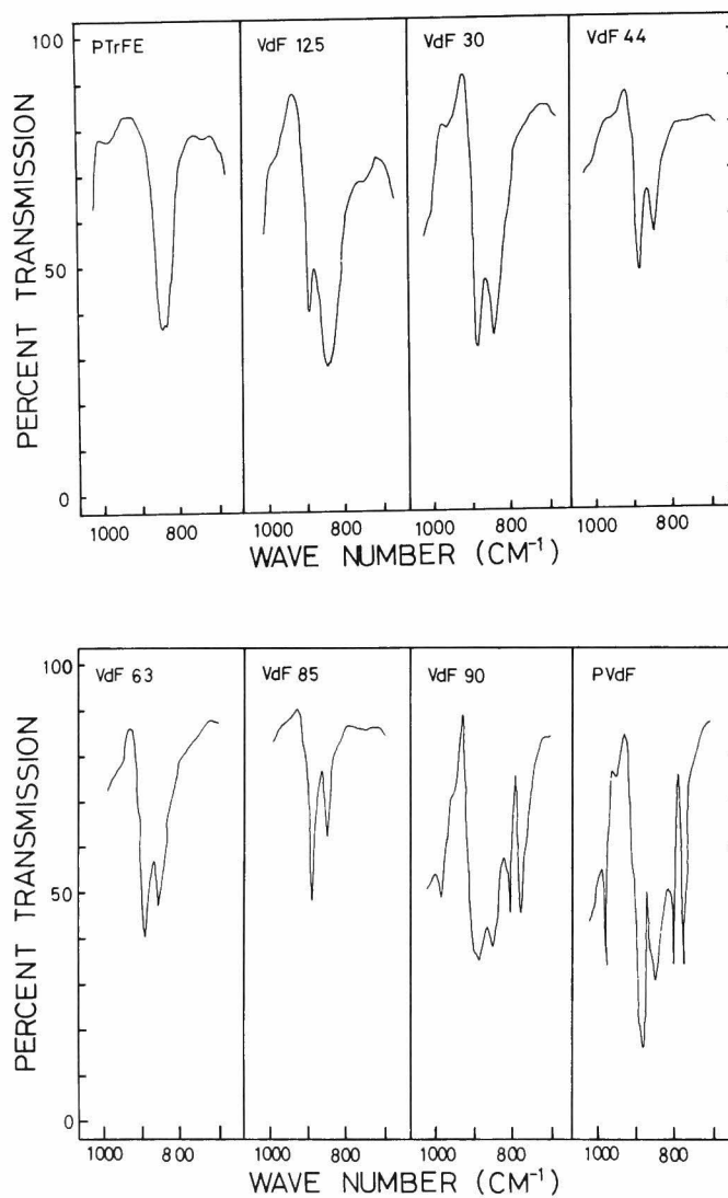
Figure 7. Infrared spectra of TrFE-VdF copolymers in the region from 650 to 1050 \text{cm}^{-1} .
