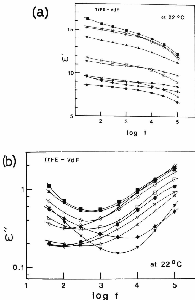
Figure 2. Frequency dependence of \epsilon' (a) and \epsilon'' (b) of the TrFE-VdF copolymer, at 22 °C.
