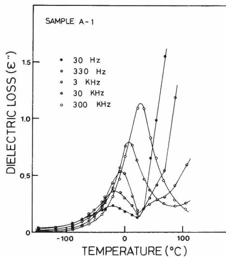
Figure 6. Temperature dependence of dielectric loss \epsilon'' for PTrFE (sample A-1-l).
