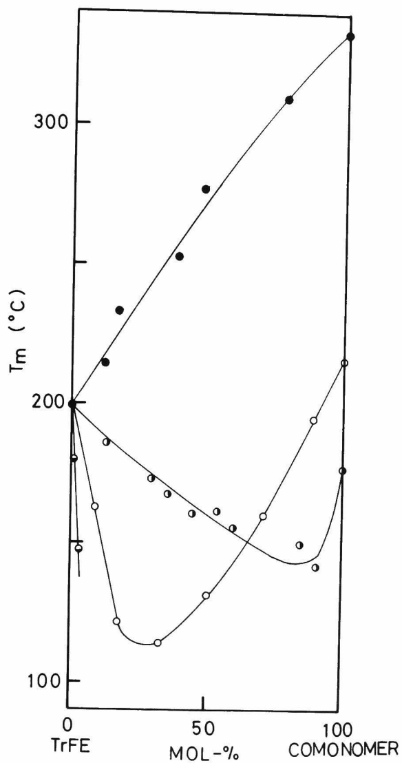
Figure 1. Change of melting temperature T_m with polymer composition: ●, TrFE-VdF; ●, TrFE-TFE; ○, TrFE-CTFE; and ●, TrFE-HFP.
