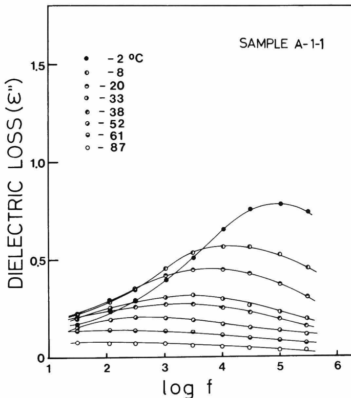
Figure 10. Frequency f dependence of dielectric loss \epsilon'' for PTrFE (sample A-1-1) at various temperature.
