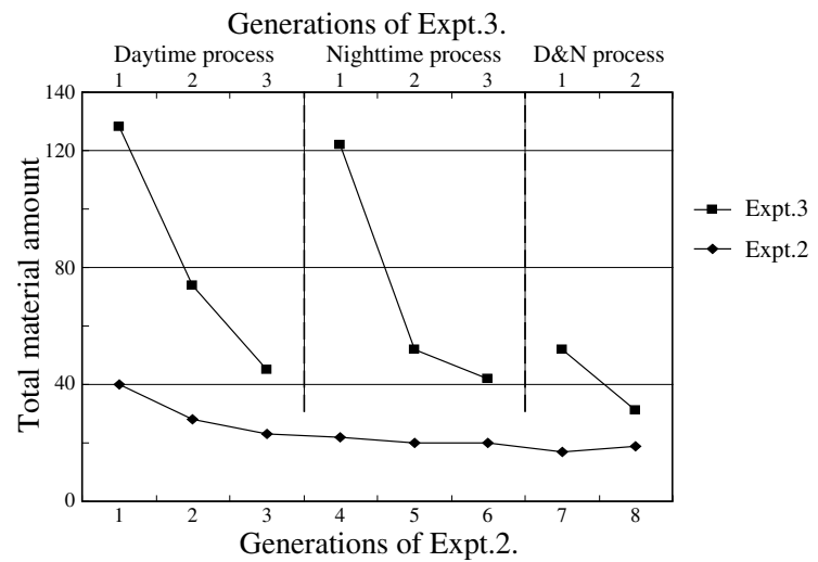
Figure 2-15 Evolution of material amount in each generation in experiments 2 and 3
