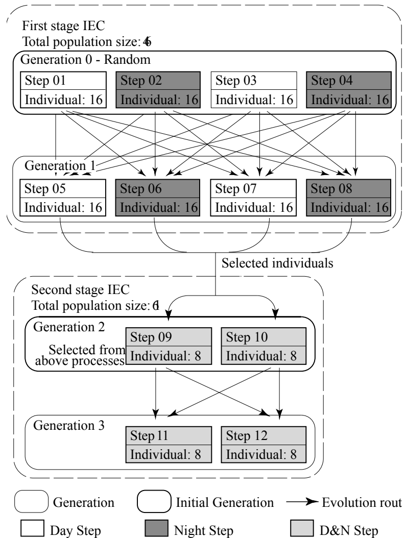
Figure 3-2 The IEC flow
