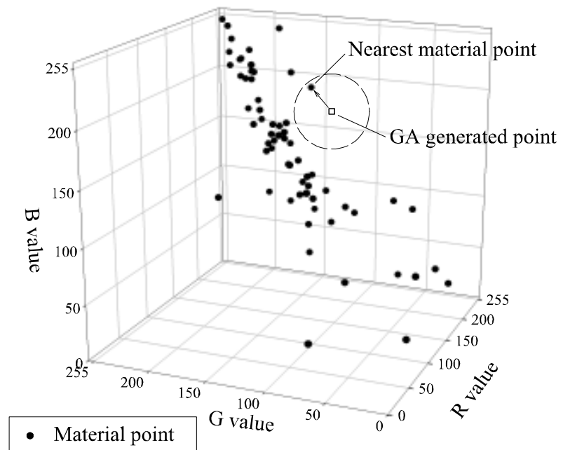
Figure 2-2 Material samples and gene relocation in RGB space.
