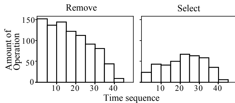
Figure 4-10 Frequency of “remove” and “select” along time sequence (02M, 03F, 04F, 07F)
