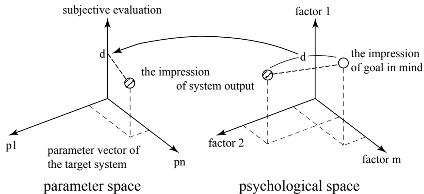
Figure 1-2 Psychological distance of user's target image and design alternative in psychological space become the fitness axis of a feature parameter space where computer search for global optimum in an IEC system (Tagaki, 2001) 5)
