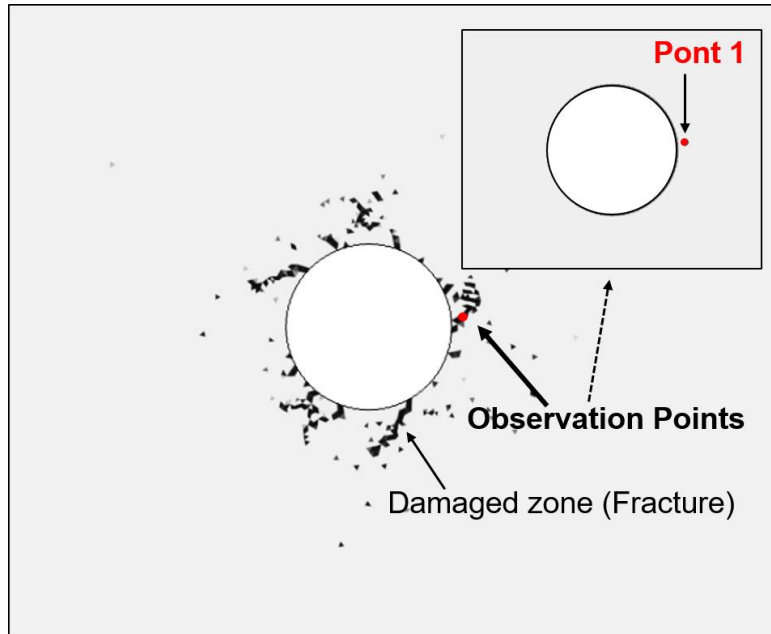
Fig. 17 Specific observation points close to cavity. The damaged zone is obtained after the completion of the excavation analysis. Point 1 is set within the predicted damaged zone.
