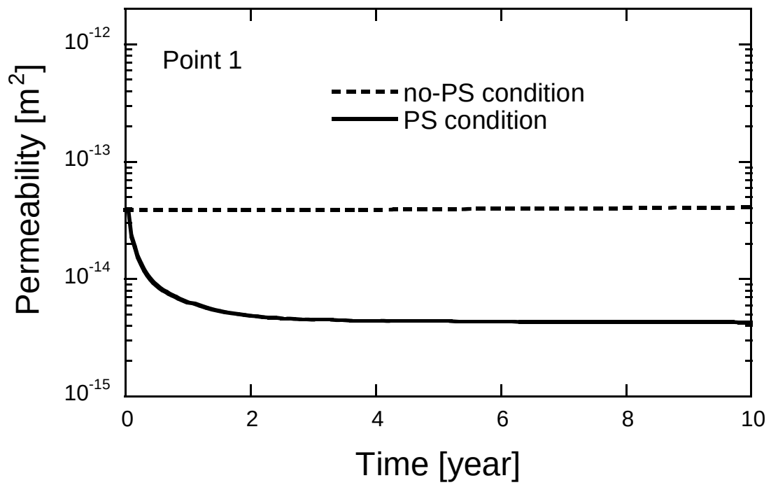
Fig. 19 Changes in permeability within first 10 years under no-PS condition and PS condition at observation point (Point 1) within damaged zone shown in Fig. 17 .
