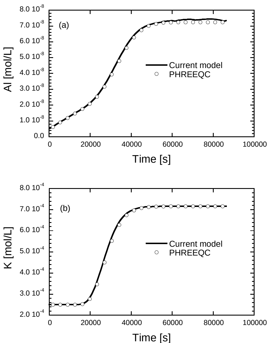
Fig. 9 Comparisons of results by proposed model versus PHREEQC solutions for evolution in concentrations of (a) Al and (b) K.
