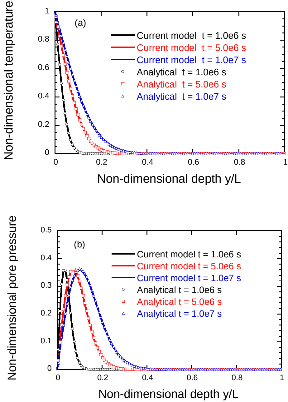
Fig. 7 Comparisons of results by proposed model versus analytical solution for (a) non-dimensional temperature and (b) non-dimensional pore pressure at different depths and at various times ( t = 1.0 \times 10^6 , 5.0 \times 10^6 , and 1.0 \times 10^7 ).
