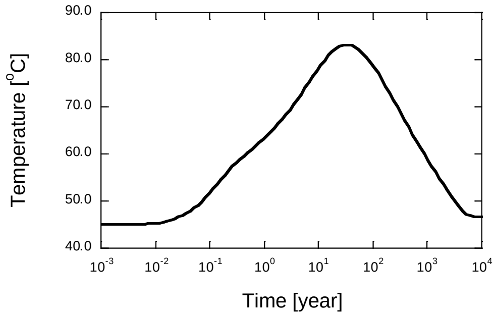
Fig. 13 Temperature depending on time T_b(t) used as boundary condition applied on periphery of cavity [49].
