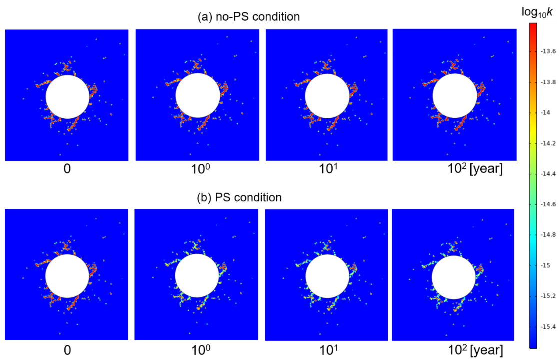
Fig. 16 Changes in permeability with time under (a) no-PS condition and (b) PS condition.
