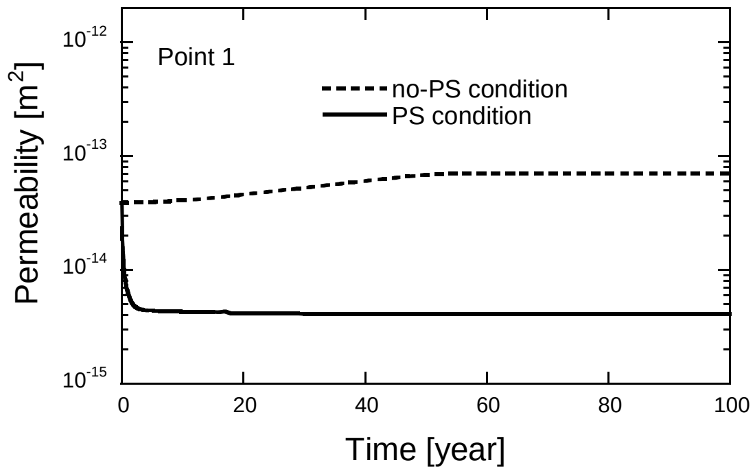
Fig. 18 Changes in permeability with time under no-PS condition and PS condition at observation point (Point 1) within damaged zone shown in Fig. 17 .
