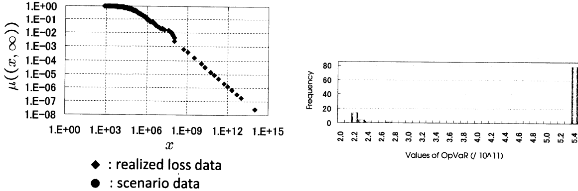
Figure 4: Histogram of 100 estimations of OpVaR.
