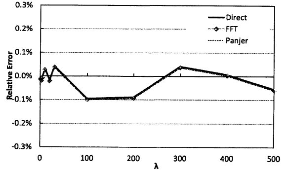
Figure 6: Relative error in the case of GPD.
