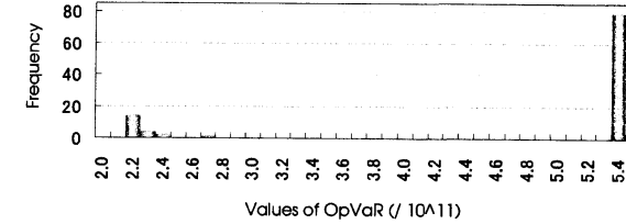
Figure 4: Histogram of 100 estimations of OpVaR.
