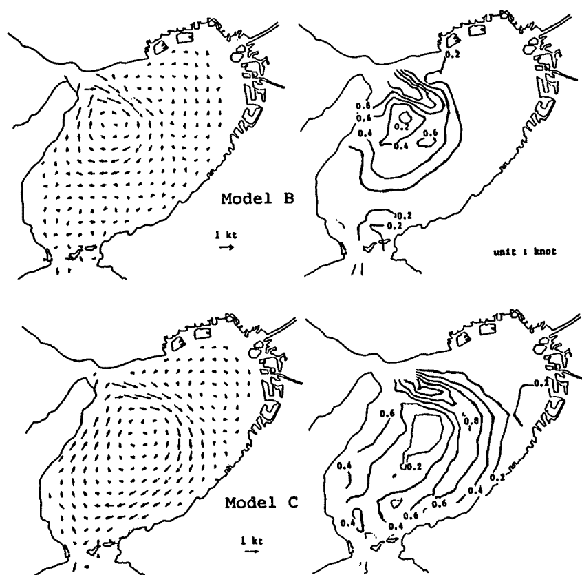
Fig. 9. Permanent flow. (Model B and C, Mean tide)
