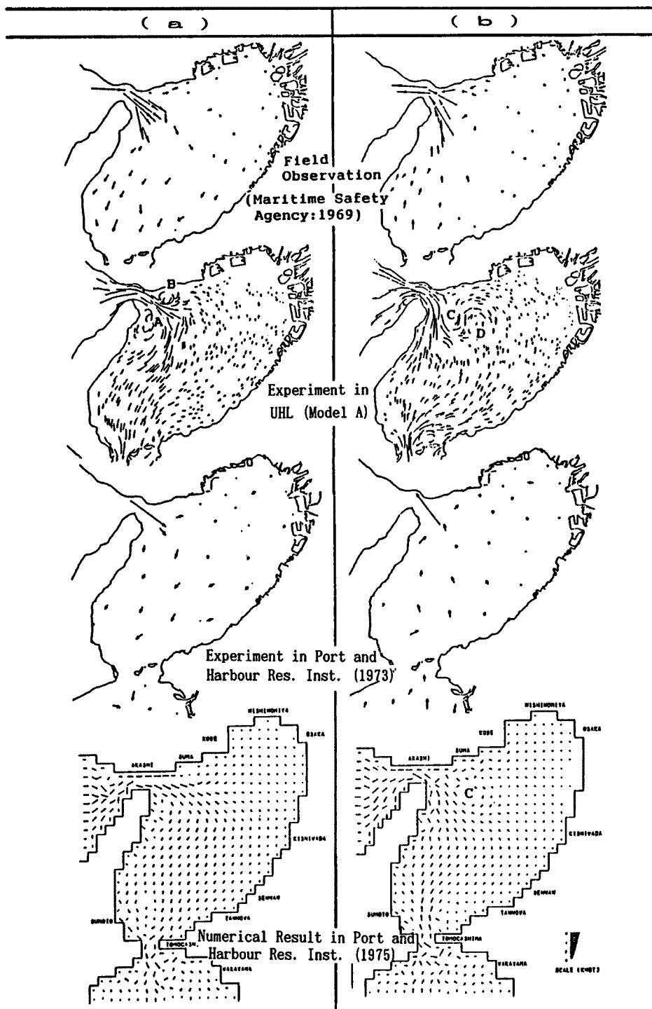
Fig. 6. Comparison of tidal currents obtained in some other models. (Spring tide) (a): Ebb tide (b): Flood tide
