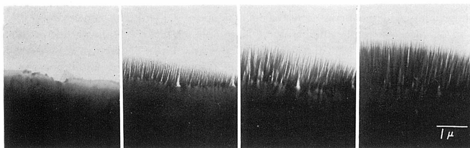
Fig. 3. Crystal growth on the surface of the \text{Li}_2\text{O} \cdot 3\text{SiO}_2 glass.
