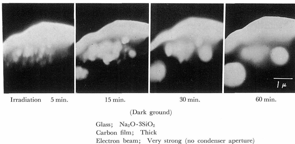
Fig. 10. Bubble formation in a glass fragment by electron bombardment.
