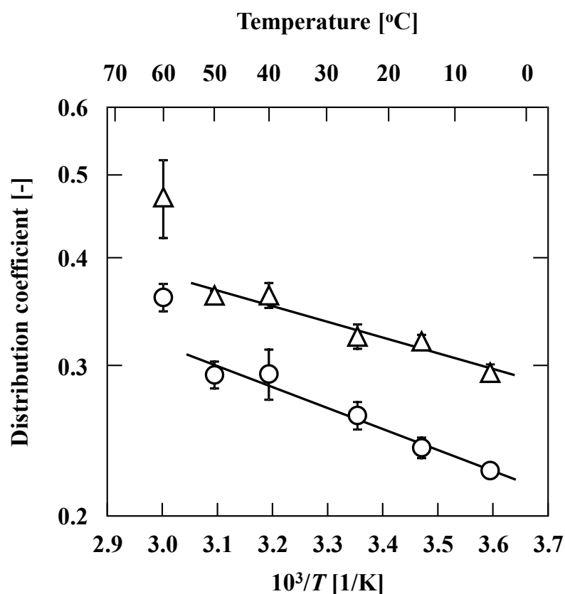
Fig. 2.4. Temperature dependence of distribution coefficient of fructose into Koshihikari (circles) and Habutaemochi (triangles). Data is represented as mean \pm standard deviation for measurements at five different concentrations.
