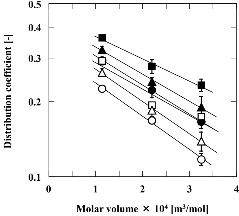
Fig. 2.3. Estimation of swelling pressures of Koshihikari (open symbols) and Habutaemochi (closed symbols) from the distribution coefficients of saccharides into rice at 5°C (circles), 25°C (triangles), and 50°C (squares).
