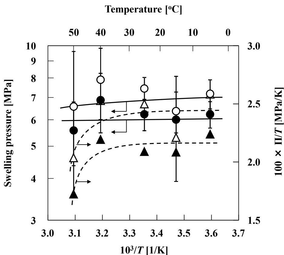
Fig. 2.5. Temperature dependence of swelling pressure (circles) and \Pi/T value (triangles) for Koshihikari (open symbols) and Habutaemochi (closed symbols). Error bars for swelling pressure represent 90% confidence interval.
