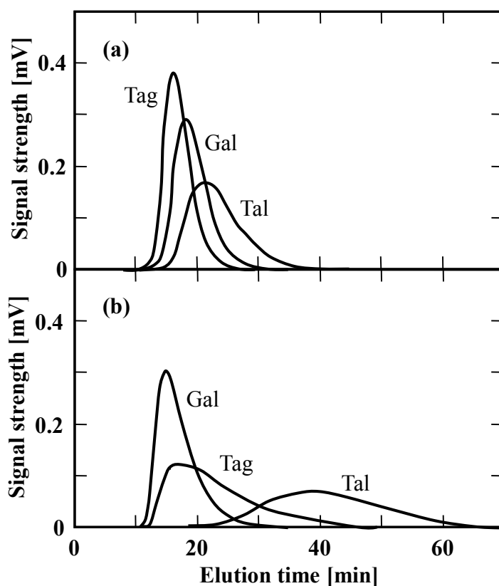
Fig. 4.1. Elution profiles of galactose (labeled Gal), tagatose (Tag) and talose (Tal) for the resins in the (a) K^+ and (b) Ca^{2+} forms with 8% DVB content at 30°C. The eluent used was water.
