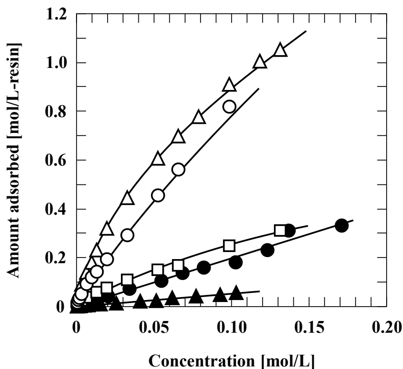
Fig. 3.2. Adsorption isotherms of methylparaben (○), vanillin (△), isovanillin (□), coumarin (●), and caffeine (▲) onto the chromatographic organic monolith at 24°C.
