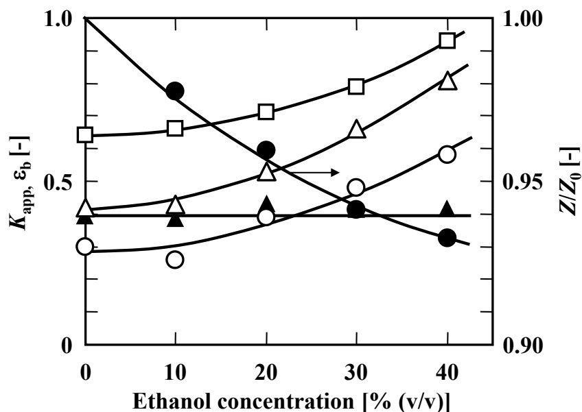
Fig. 4.2. Relative bed height, Z/Z_0 (●), bed voidage, \epsilon_b (▲), and the K_{app} values for galactose (△), tagatose (○) and talose (□) for eluent containing different ethanol content for the resin in the K^+ form with 8% DVB content at 30°C.
