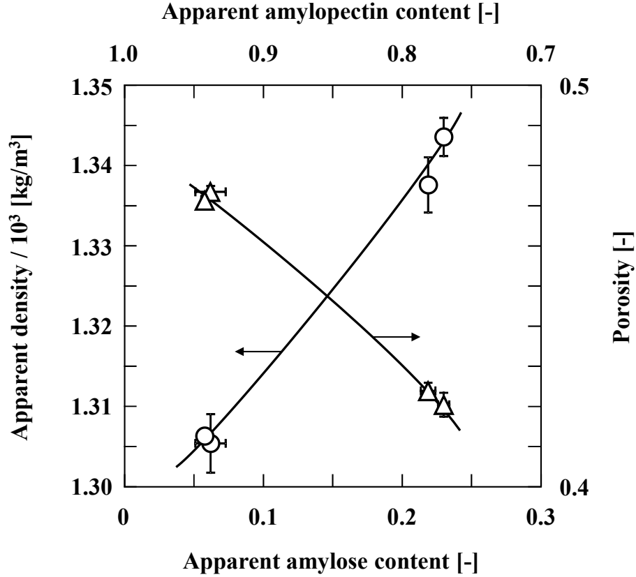
Fig. 2.2. Effects of apparent amylose content on apparent density (circles) and porosity (triangles) of rice at 25°C. Symbols from left to right represent Kitayukimochi, Habutaemochi, Yumepirika and Koshihikari, respectively. Apparent amylose content was measured in duplicate, and results are represented as mean \pm standard deviation.
