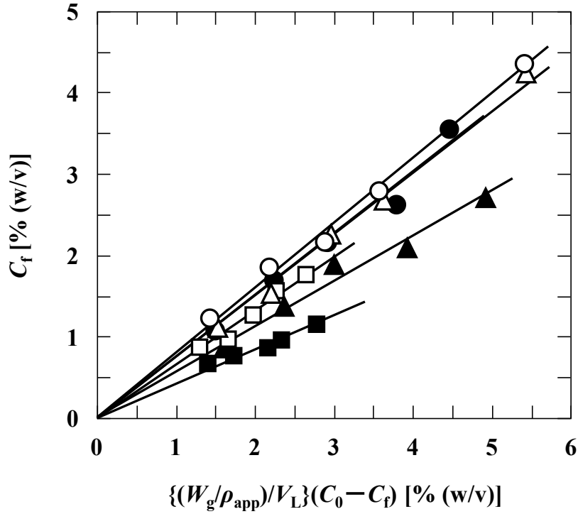
Fig. 1.2. Relationship between C_f and [(W_g/\rho_{app})/V_L] \cdot (C_0 - C_f) for ethylene glycol ( \circ , \bullet ), glucose ( \triangle , \blacktriangle ), and raffinose ( \square , \blacksquare ) at 25°C (open symbols) and 50°C (closed symbols).
