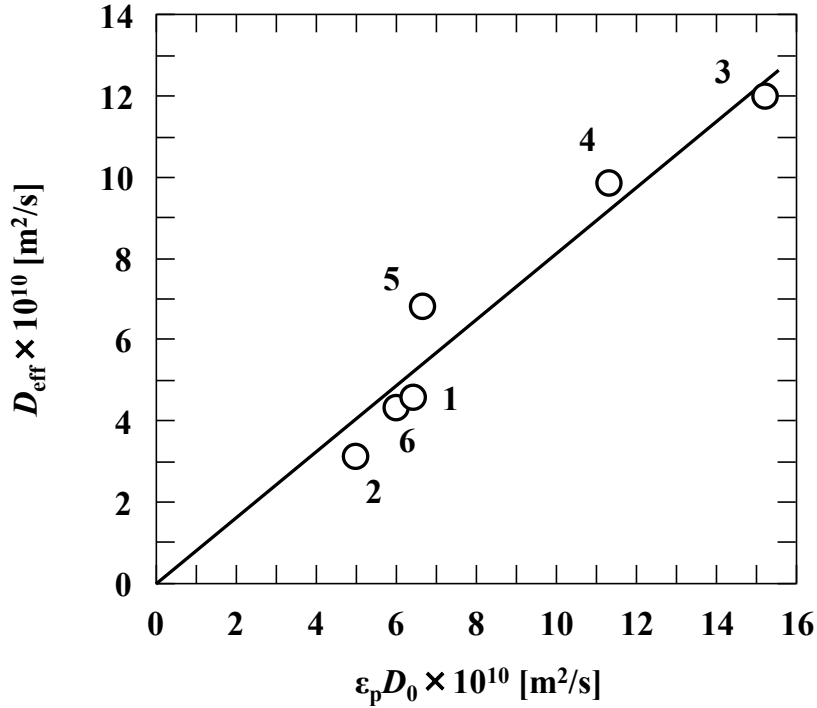
Fig. 1.7. Relationship between D_{\text{eff}} and \epsilon_p D_0 . Numbers represent the seasoning compounds 1: glucose, 2: sucrose, 3: NaCl, 4: acetic acid, 5: monosodium glutamate, and 6: vanillin.
