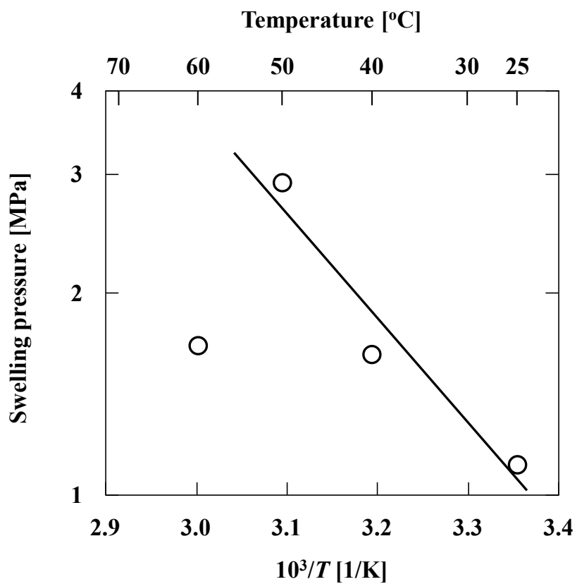
Fig. 1.4. Temperature dependence of the swelling pressure of starch gel.
