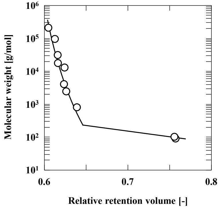
Fig. 3.1. Estimation of chromatographic organic monolith porosity by inverse size-exclusion chromatography.
