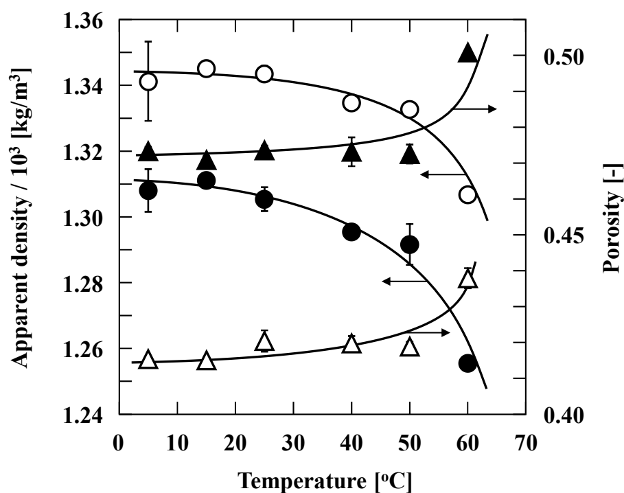
Fig. 2.1. Temperature dependence of apparent density (circles) and porosity of rice (triangles). Symbols represent apparent density of Koshihikari (open symbols) and Habutaemochi (closed symbols). Values obtained from triplicate measurements are represented as mean \pm standard deviation.
