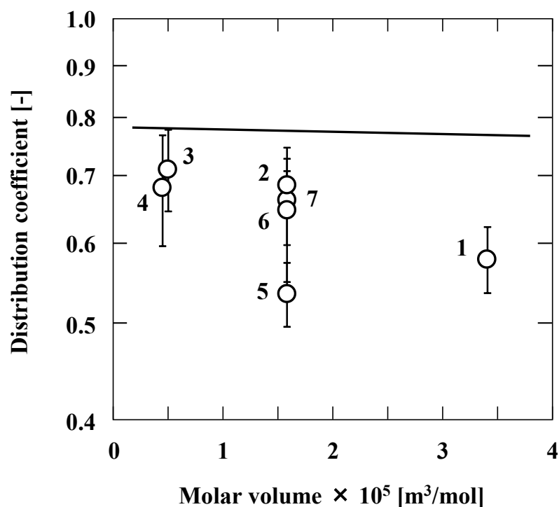
Fig. 1.6. Distribution coefficients of electrolytes at 25°C. Numbers represent the electrolytes used: 1: LiCl, 2: NaCl, 3: KCl, 4: CsCl, 5: NaF, 6: NaBr, and 7: NaI. The values are represented as mean \pm SD.
