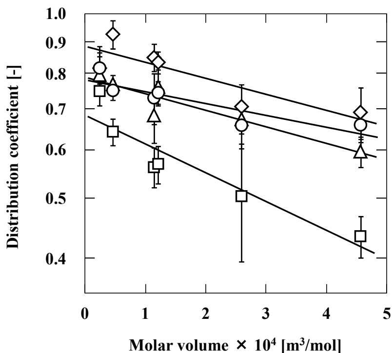
Fig. 1.3. Estimation of swelling pressure of the starch gel at 25°C (○), 40°C (△), 50°C (□), and 60°C (◇) using Eq. (1.3). The solutes used were ethylene glycol, glycerol, fructose, glucose, sucrose, and raffinose.
