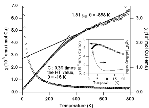
Figure 2. Temperature dependence of magnetic susceptibility of \text{La}_4\text{Cu}_3\text{MoO}_{12} below 800 K. The solid lines correspond the fit to the Curie-Weiss law. The inset shows the data taken at 0.1 T.
