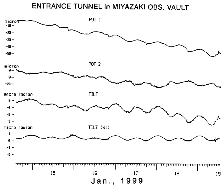
Fig.5 Record of test observation at entrance tunnel in Miyazaki observatory vault by type III instrument. (from top to bottom: POT1 level, POT2 level, tilt and record of routine tilt observation in the same direction in the observatory by type I instrument.)
