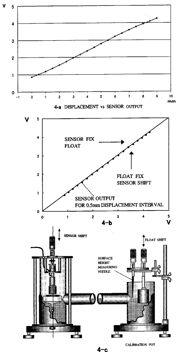
Fig.4 Calibration of displacement sensor and test of effect of magnetic attraction in alignment system.
