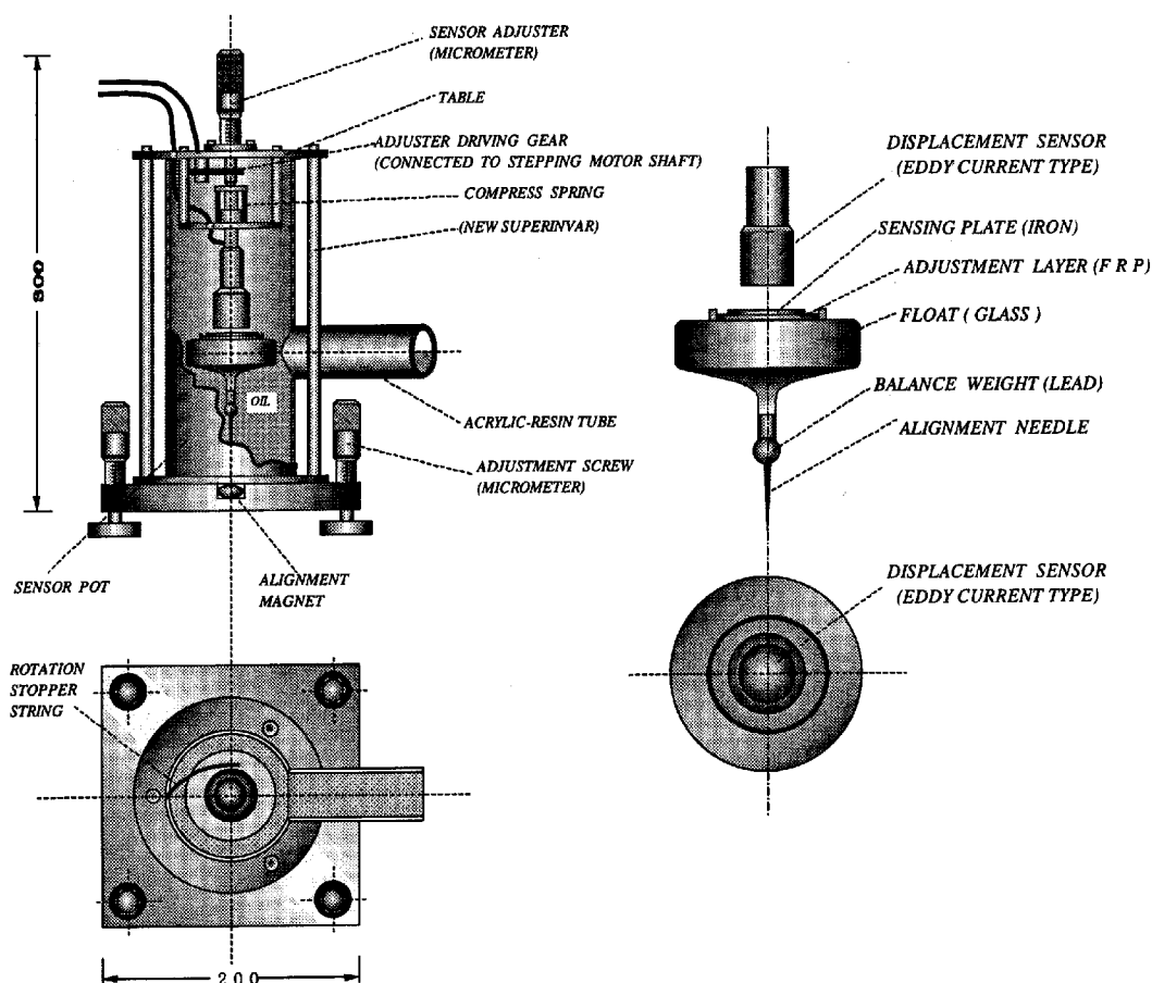
Fig.3 Newly designed half-filled water-tube tiltmeter without float suspension mechanism. (type III)
