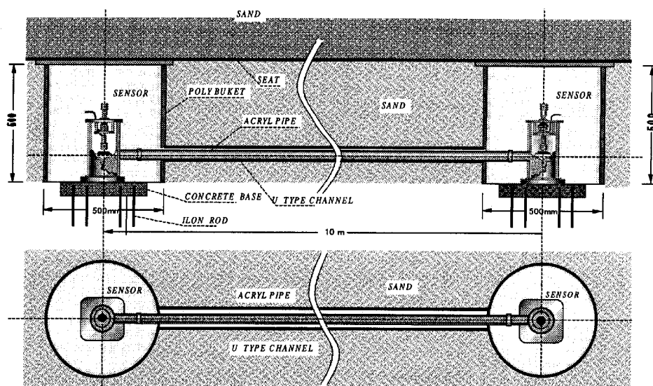
Fig.6 Schematic view of installation of type III instrument in ground surface trench.
