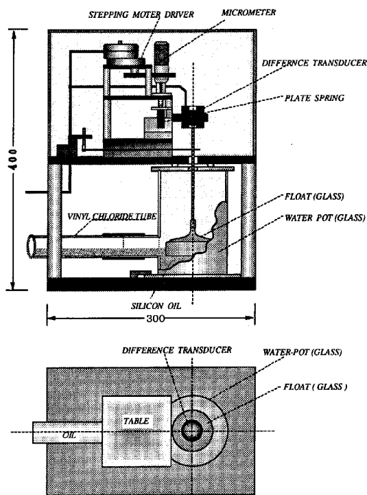
Fig.2 Type II water-tube tiltmeter. (half-filled type)
