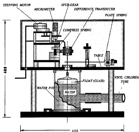
Fig.1 Type I water-tube tiltmeter. (full-filled type)
