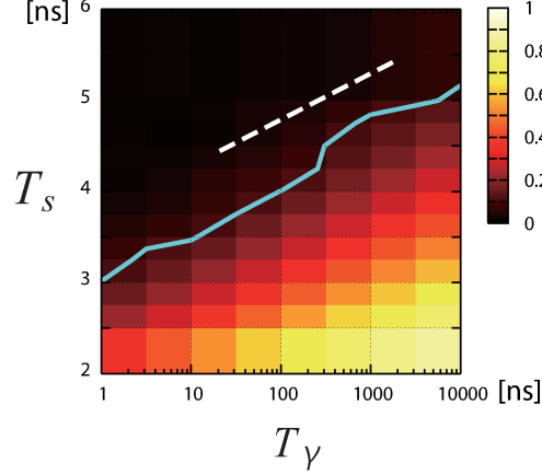
Fig. 1: The correlation coefficient C(T_\gamma, T_s) for temporally correlated noise. The light blue curve is defined by C(T_\gamma, T_s) = 0.1 . The white broken line represents T_s \propto 0.5 \log T_\gamma as a reference of the discussion in the appendix A.
