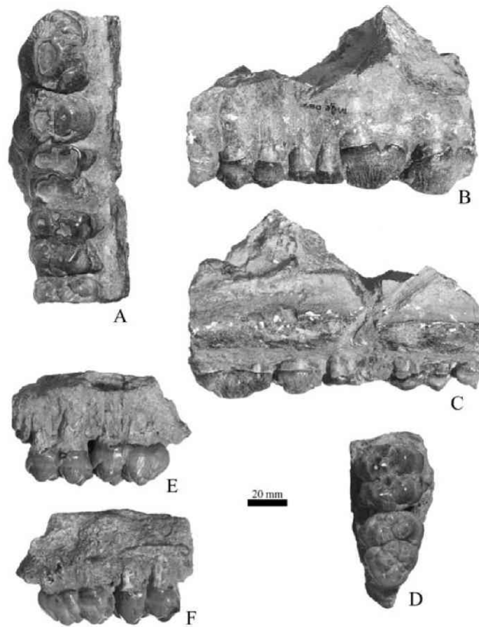
Figure 4. Upper cheek teeth of Tetraconodon sp. cf. T. magnus . A-C , YUDG-Mge 089, a right maxillary fragment with P^3 – M^2 with anterior half of M^3 : A , occlusal view; B , buccal view; C , lingual view. D-F , YUDG-Mge 091, a left maxillary fragment with M^{2-3} : D , occlusal view; E , buccal view; F , lingual view.
