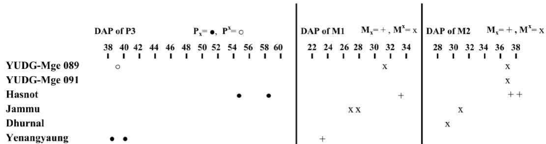
Figure 6. Comparisons of the anteroposterior length (=DAP; mm) of the P^3/3 , M^1/1 and M^2/2 in Tetraconodon . The localities are in approximate stratigraphical order from older (bottom) to younger (top); T. minor , the type locality Yenangyaung; T. intermedius (= T. mirabilis ), Dhurnal and the type locality Jammu; T. magnus , the type locality Hasnot (after Made, 1999: fig. 7). Closed and open circles indicate lower and upper third premolars, respectively. Cross and X indicate lower and upper molars, respectively. The lengths of M^1 and M^2 of Tetraconodon sp. cf. T. magnus are larger than those of T. intermedius .
