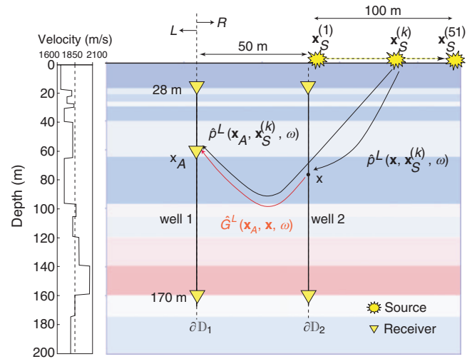
Figure 1. Velocity model and source-receiver configuration used for numerical modeling. There are 72 receivers at 2-m intervals in each borehole and 51 sources ( \mathbf{x}_S^{(1)} to \mathbf{x}_S^{(51)} ) at the surface. The expressions \mathbf{x}_S^{(k)} , \mathbf{x} , and \mathbf{x}_A represent the source and the two observation locations as used in equations 5 and 7, whereas \partial D_1 and \partial D_2 indicate the chosen position of the boundaries from equation 6. The expression \hat{p}^L(\mathbf{x}_A, \mathbf{x}_S^{(k)}, \omega) is the acoustic wavefield observed at receiver position \mathbf{x}_A in well 1 from a physical source at the surface at \mathbf{x}_S^{(k)} . The expression \hat{p}^L(\mathbf{x}, \mathbf{x}_S^{(k)}, \omega) is the acoustic wavefield observed at receiver position \mathbf{x} in well 2 from the same physical source at \mathbf{x}_S^{(k)} . The expression \hat{G}^L(\mathbf{x}_A, \mathbf{x}, \omega) represents the crosswell Green's function at receiver position \mathbf{x}_A in well 1, assuming that receiver \mathbf{x} in well 2 is the virtual source position.
