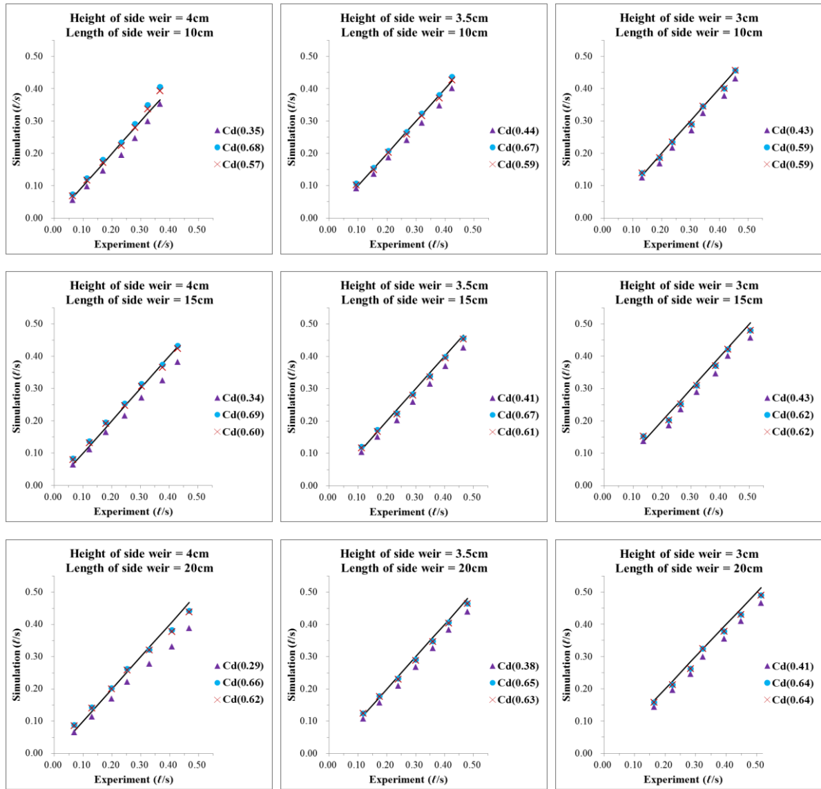
Fig. 9 Suitable discharge coefficients under different weir conditions
