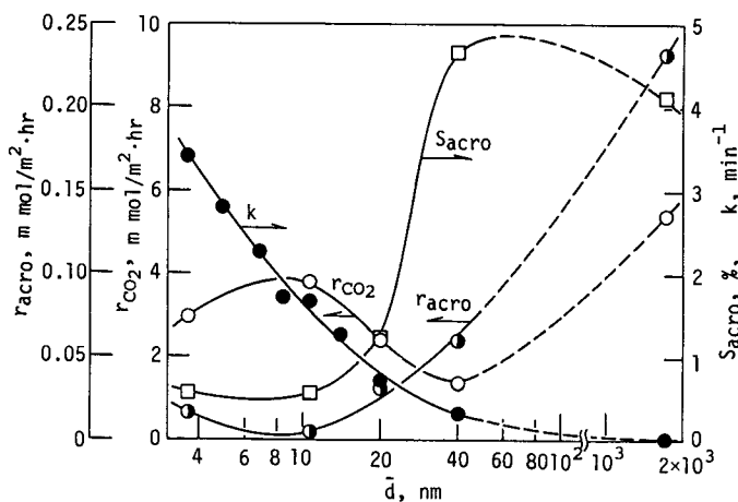
Fig. 5. Effect of copper particle size( \bar{d} ) on the \text{C}_3\text{H}_6 oxidation and initial rate of stoichiometric Cu oxidation( k ).
