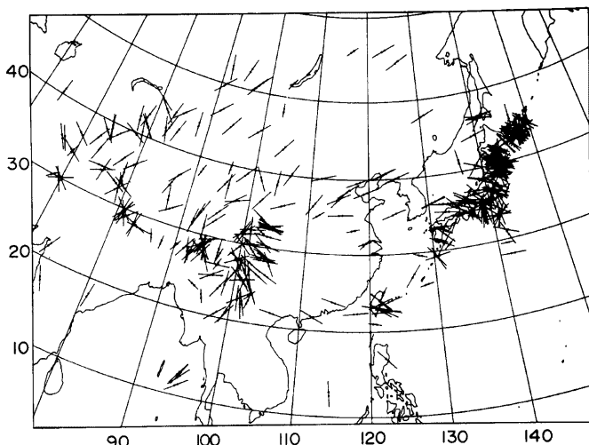
Fig. 4 Distribution extensional axes. Length of arrows indicates same as in Fig. 3.
