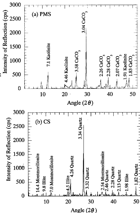
Fig. 9 X-ray diffraction patterns of PMS and CS
