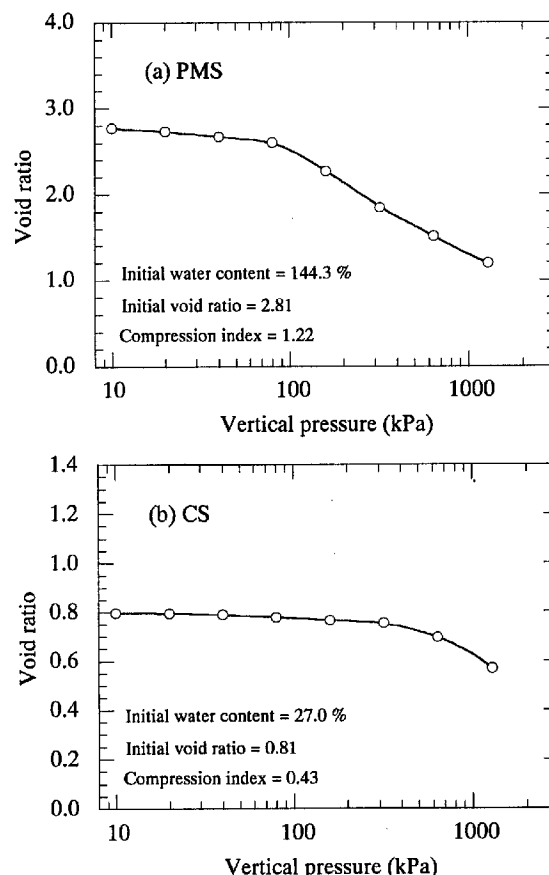
Fig. 5 Consolidation properties of PMS and CS
