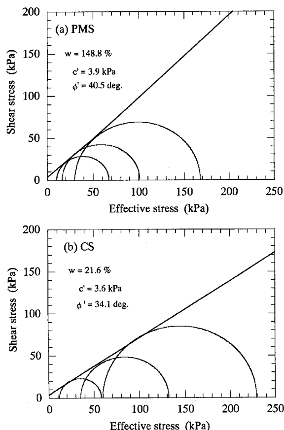
Fig. 4 Shear strength of PMS and CS
