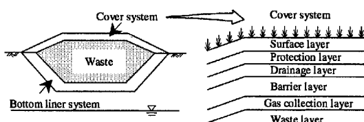
Fig. 1 Components of landfill containment and cover systems
