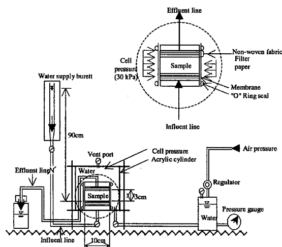
Fig. 2 Schematic diagram of hydraulic conductivity experimental setup
