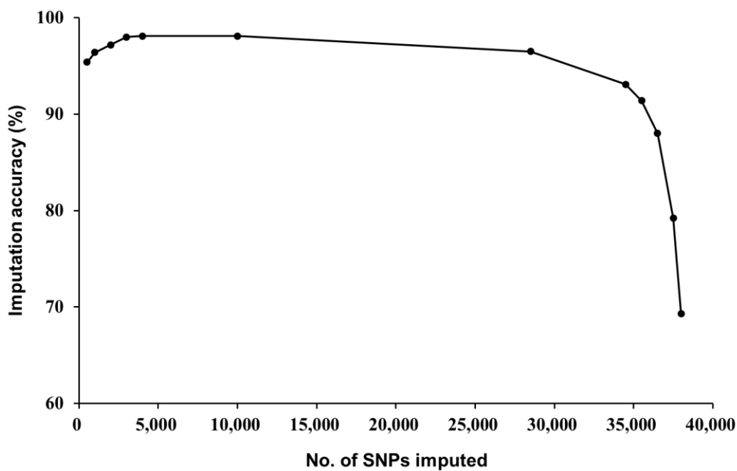
Figure 3-5. Imputation accuracy against SNP panel density.
