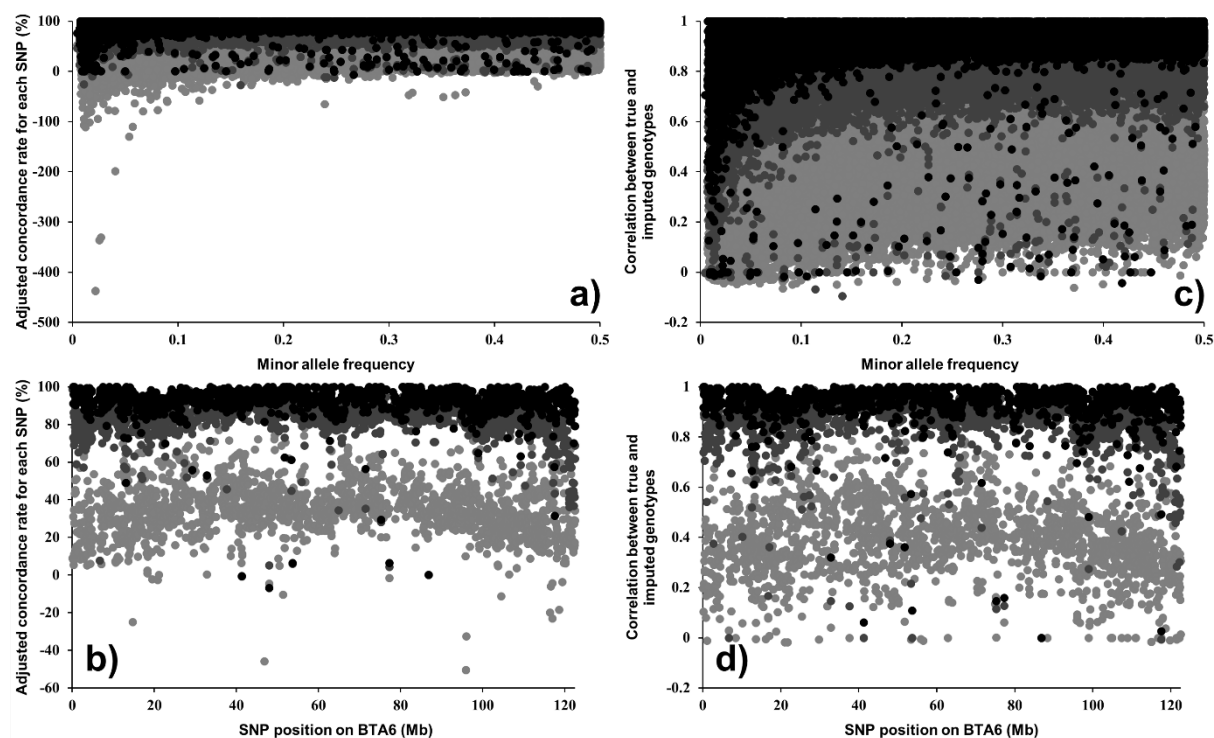
Figure 3-7. Adjusted concordance rates for each SNP and the correlation between true and imputed genotypes against minor allele frequency—(a) and (c), respectively—and against physical position on BTA6—(b) and (d), respectively. Light gray, dark gray and black dots represent the results when imputed from 500, 3,000 and 10,000 SNPs selected by method 1, respectively.
