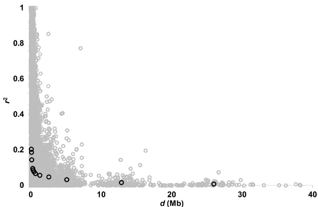
Figure 2-2. Change in mean of r^2 against mean of d (black circles), together with all values of r^2 (gray circles).
