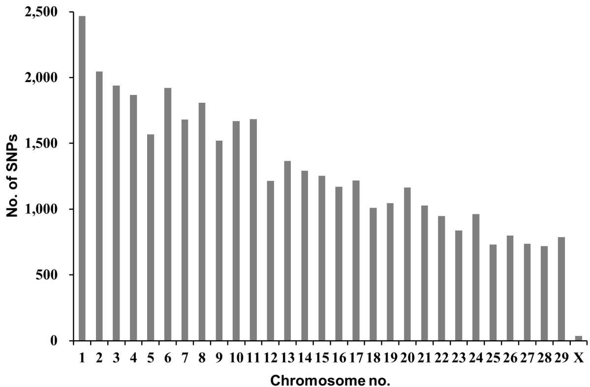
Figure 3-1. The number of SNPs on each chromosome.
