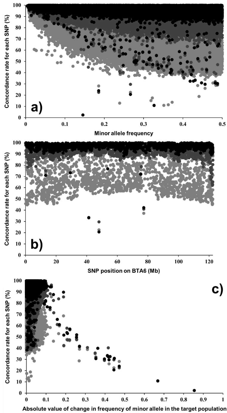
Figure 3-2. Concordance rate for each SNP ( C_{\text{SNP}} ) against minor allele frequency (a), physical position on BTA6 (b), and absolute value of change in the frequency of minor alleles in the target population (c). Light gray, dark gray and black dots represent the results when imputed from 500, 3,000 and 10,000 SNPs selected by method 1, respectively.
