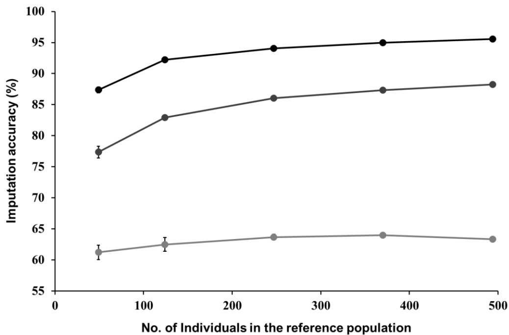
Figure 3-6. Imputation accuracy against reference population size. Values are expressed as mean \pm SD for 5 replicates. Light gray, dark gray and black dots represent the results when imputed from 500, 3,000 and 10,000 SNPs selected by method 1, respectively.
