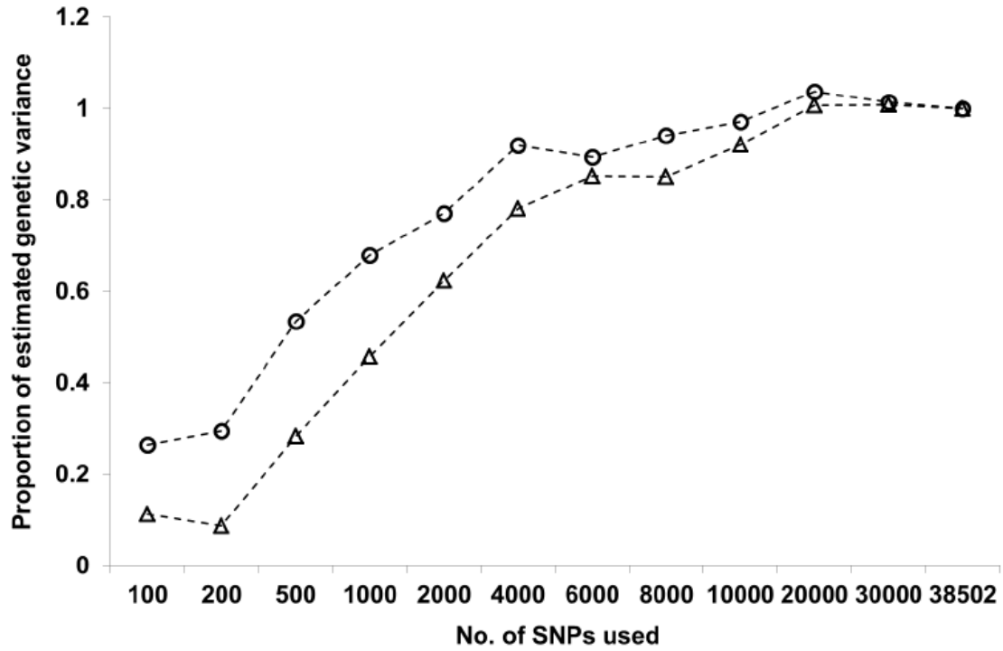
Figure 2-4. Changes in proportions of estimated genetic variances in model 1, with increasing density of SNPs used to construct G matrix. Circles: carcass weight; triangle: marbling score.
