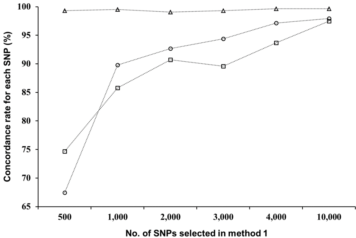
Figure 3-3. Changes in the concordance rates ( C_{\text{SNP}} ) for each of the 3 SNPs reported by Nishimura et al. (2012) against the number of equally spaced SNPs used. circle: SNP Hapmap46986-BTA-34282 ; triangle: SNP Hapmap26308-BTC-057761 ; square: SNP BTA-52694-no-rs .
