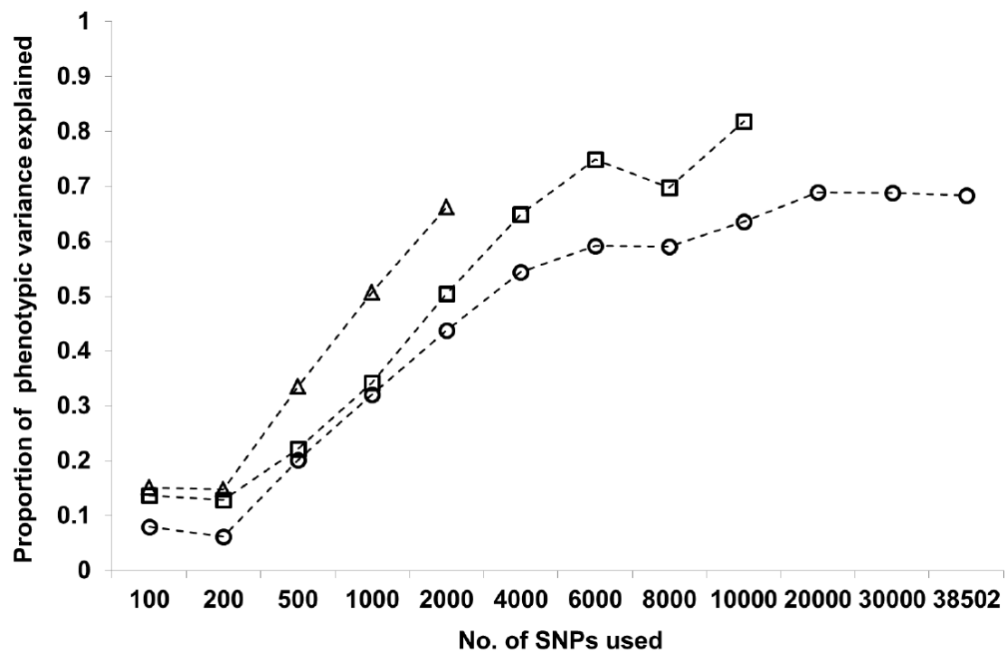
Figure 2-6. Changes in proportions of phenotypic variances explained with model 1 and 2 for marbling score, with increasing density of SNPs used to construct G matrix. Circles: model 1; triangle: model 2 (binary); square: model 2 (categorical with 11 categories).
