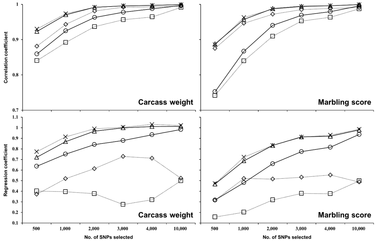
Figure 4-2. Changes in correlation coefficients (above) between, and linear regression coefficients (below) for, GEBVs for carcass weight and marbling score. Circles and triangles with solid lines represent the correlation coefficients between GEBVs obtained using \mathbf{G}_{\text{ALL}} based on the actual genotypes of all available SNPs and GEBVs using \mathbf{G}_{\text{SUB}} based on the actual genotypes of only selected SNPs as well as GEBVs using \mathbf{G}_{\text{IMP}} based on the imputed genotypes in model 1, respectively. Crosses, squares and rhombuses with dotted lines represent the coefficients between GEBVs obtained with model 1 using the actual genotypes of all the available SNPs and GEBVs, \hat{\mathbf{g}}_1 + \hat{\mathbf{g}}_2 , \hat{\mathbf{g}}_1 and \hat{\mathbf{g}}_2 from model 2, which were obtained with \mathbf{G}_2 constructed using the imputed genotypes of the corresponding SNPs. For linear regression, circles and triangles with solid lines represent the coefficients where the independent variable was GEBVs obtained using the actual genotypes of all the available SNPs and the dependent variables were GEBVs obtained using the actual genotypes of only selected SNPs and using the imputed
