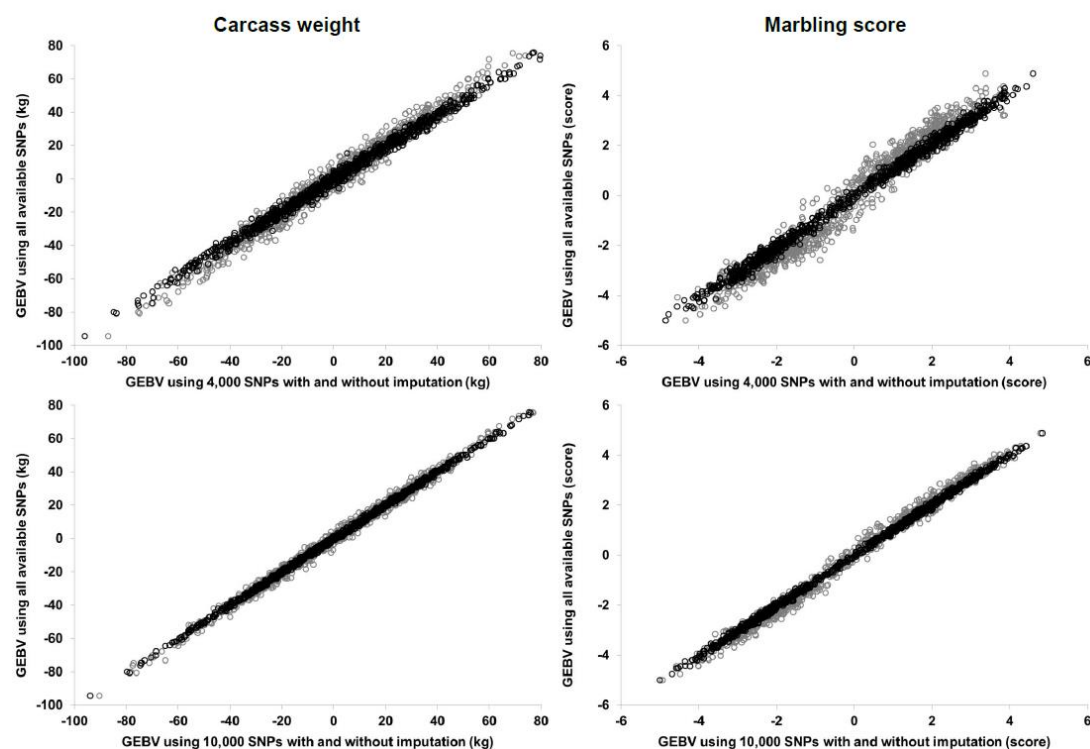
Figure 2-5. Scatter plots for GEBVs obtained with model 1 using 4,000 (top panels) or 10,000 (bottom panels) SNPs and those using all available SNPs, for carcass weight (left panels) and marbling score (right panels) with and without imputation. Black circles: with imputation; gray circles: without imputation.
