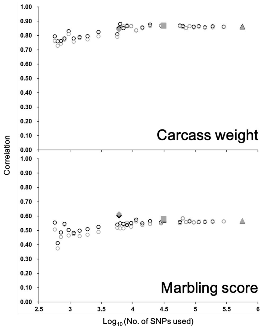
Figure 5-2. Changes in the prediction accuracy assessed as the correlation between the genomic estimated breeding values and the records corrected by all the fixed effects estimated in the official genetic evaluation using pedigree data for animals in the validation population, divided by the squared root of estimated heritability. Triangles, squares and rhombuses show the results obtained using HD, 50K and LD SNP sets, respectively. Circles represent the results using lower-density SNP subsets. Black and gray show the results using G matrices of VanRaden (2008) and the modification of the matrix of Yang et al. (2010), respectively.
