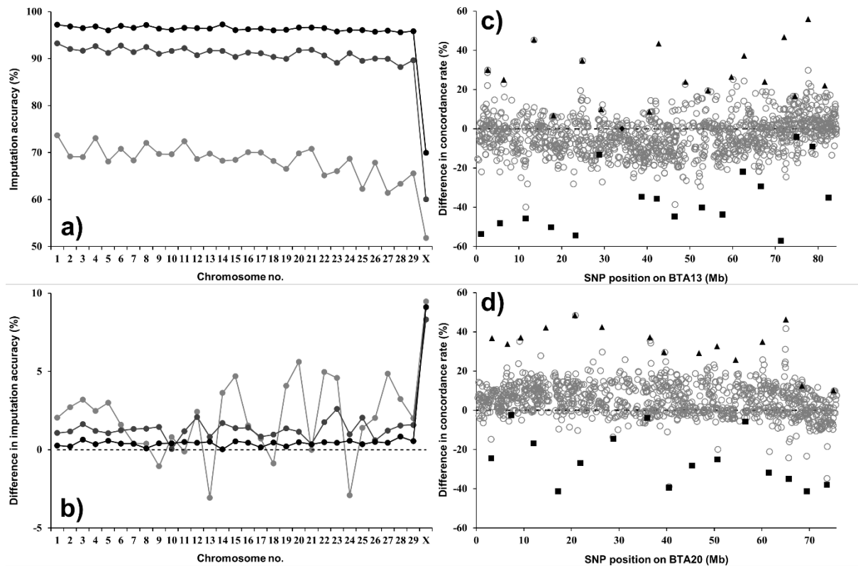
Figure 3-4. Imputation accuracy at the chromosome level using method 1 (a), the difference between methods 1 and 2 in imputation accuracy (b), the difference between methods 1 and 2 in concordance rate for each SNP ( C_{\text{SNP}} ) of the SNPs on BTA13 (c) and BTA20 (d). The axis of ordinate in (b), (c) and (d) represents the difference between the values obtained by method 2 and the corresponding values obtained by method 1. For (a) and (b), light gray, dark gray and black dots represent the results when imputed from 500, 3,000 and 10,000 SNPs selected by method 1, respectively. For (c) and (d), gray circle: SNP not selected by either methods 1 or 2; black triangle: SNP selected by method 1 but not method 2; black square: SNP selected by method 2 but not method 1; black rhombus: SNP selected by both methods 1 and 2.
