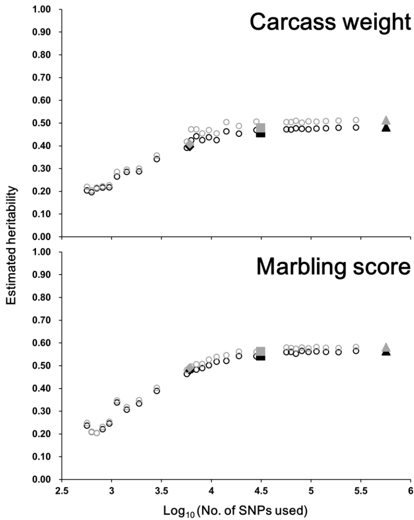
Figure 5-1. Changes in the value of estimated heritability. Triangles, squares and rhombuses show the results obtained using HD, 50K and LD SNP sets, respectively. Triangles, squares and rhombuses show the results obtained using HD, 50K and LD SNP sets, respectively. Circles represent the results using lower-density SNP subsets. Black and gray show the results using G matrices of VanRaden (2008) and the modification of the matrix of Yang et al. (2010), respectively.
