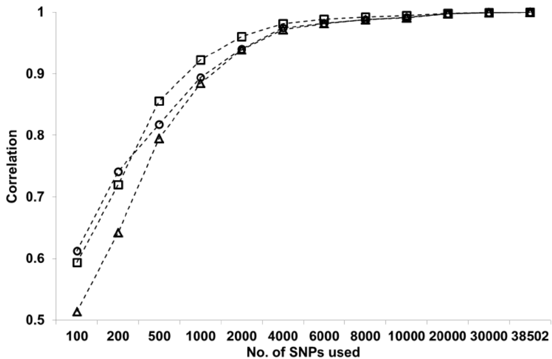
Figure 2-3. Changes in r_D , r_N and r_A with increasing density of SNPs used to construct G matrix. Circles: r_D ; triangles: r_N ; squares: r_A .
