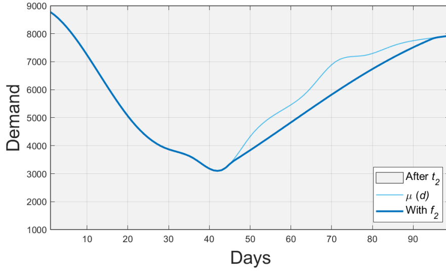
Figure 7.7 \mu and \tilde{\mu} fitting of Cluster 4 ( \beta_r = 0.042 )
