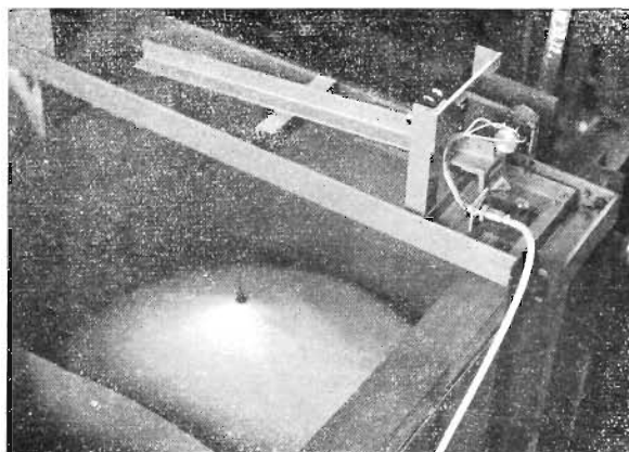
Photo. 3. Water level transmitter for automatic control.
