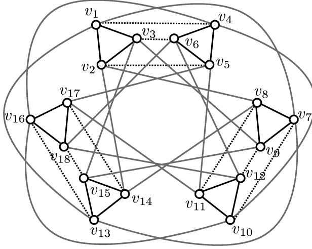
Figure 1. A counterexample for (2, 4) -boundedness of P_N(I)
