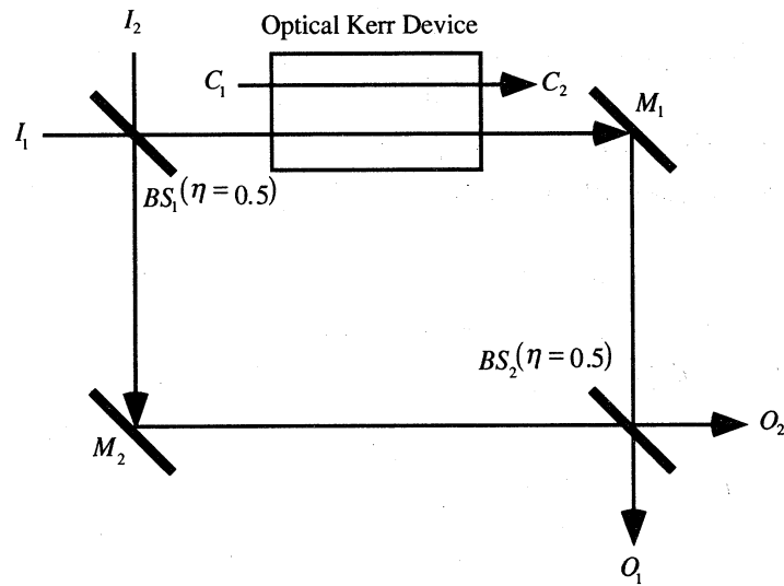
Fig 2.1 FTM gate
