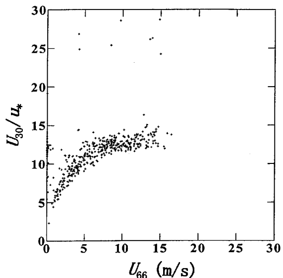
Fig. 4 U_{30}/u_* shown as a function of U_{66} .
