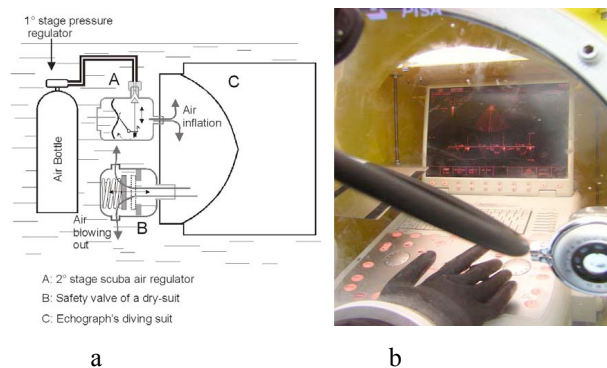
Fig. 6. a: pneumatics of the Echograph housing; b: echograph operated at 5m depth
