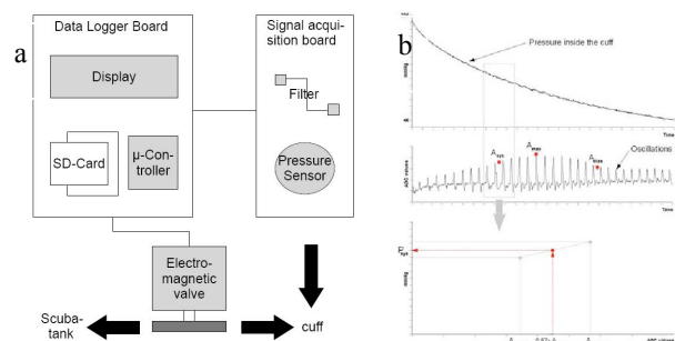
Figure 4. a: outline of the underwater blood pressure meter; b: raw data and calculation of systolic and diastolic pressures
