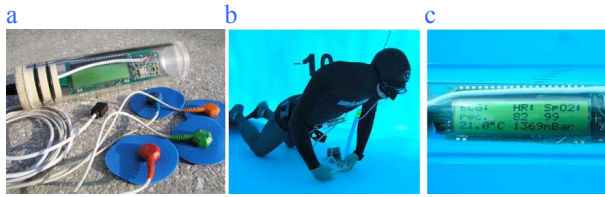
Figure 2. a: Prototype; b: breath hold diver at 10,5 mfw; c: LCD display
