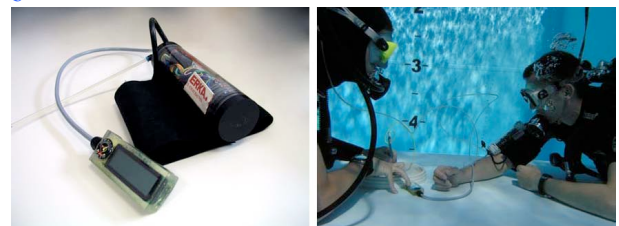
Figure 5. a: first prototype of the blood pressure meter b: tests at 4 m depth Underwater
