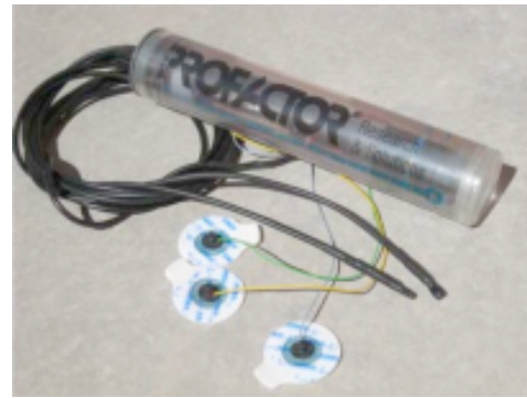
Figure 1. ECG recorder prototype housed in a lexan tube. Two temperature sensors are placed in the diving suit for continuous monitoring of the skin temperature.
