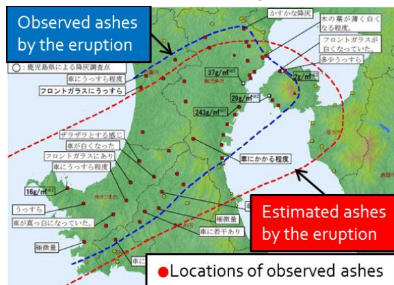
Fig. 11 Volcanic ash coluds (Observed, Blue dotted line) by the eruption of Sakurajima on April 9 (after Kagoshima Local Meteorological Observatory)
