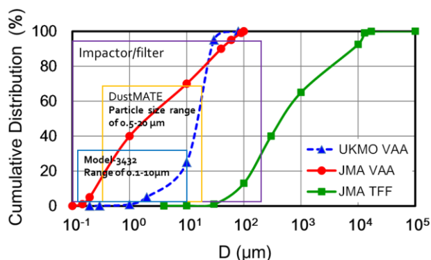
Fig.7 Component of the Eyjafjallajökull volcanic ash plume
