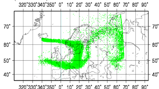
Fig. 10(b) Volcanic ash clouds, FL200/FL350
