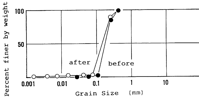
Fig. 7. Grain size distribution of the Toyoura standard sand.
