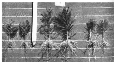
Photo. 10 Growth of the seedlings in Ca-cyanamide 120 g/m 2 plot.
