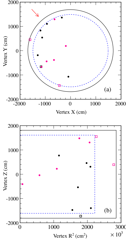
FIG. 27 (color online). (a) Two-dimensional ( x, y ) distribution of the reconstructed vertex positions of observed \nu_e candidate events. (b) Two-dimensional ( r^2 = x^2 + y^2, z ) distribution of the reconstructed vertex positions of the observed \nu_e candidate events. The arrow indicates the neutrino beam direction and the dashed line indicates the fiducial volume boundary. Black markers are events observed during Run 1 + 2, and pink markers are events from Run 3. Open squares represent events which passed all the \nu_e selection cuts except for the fiducial volume cut.
