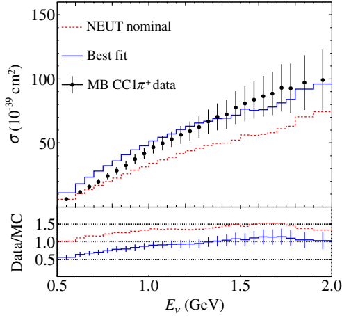
FIG. 13 (color online). The \text{CC}1\pi^+ cross section as a function of energy as measured by MiniBooNE, with the NEUT nominal and best-fit models. The treatment in the analysis of the disagreement between the best-fit NEUT and data is discussed in the text.
