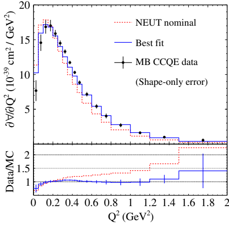
FIG. 40 (color online). The CCQE cross section as a function of Q^2 (top) as measured by MiniBooNE (points), with the NEUT nominal and NEUT at the best-fit of the MiniBooNE CCQE ( T_\mu, \cos \theta_\mu ) spectrum. Ratio of data to NEUT (bottom) for nominal (dashed line) and best fit (solid line).
