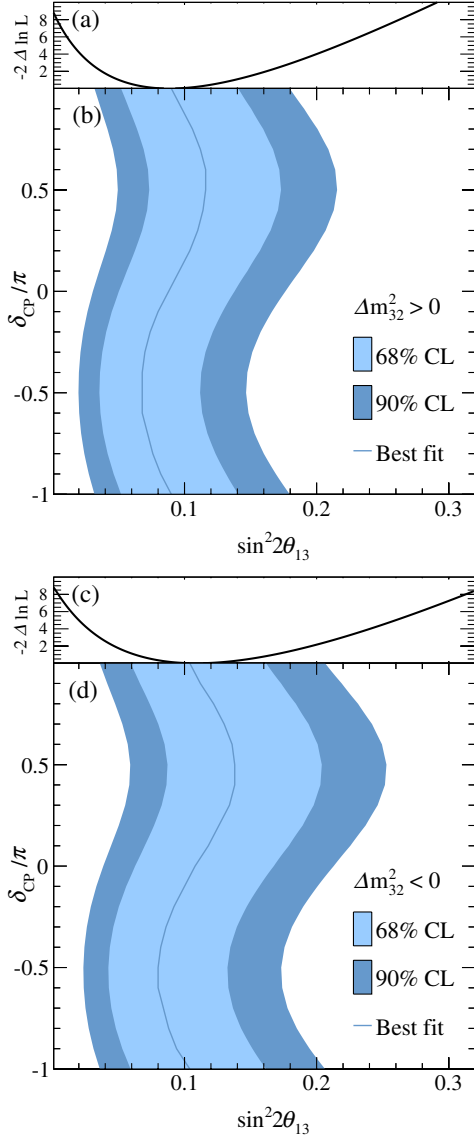
FIG. 36 (color online). The 68% and 90% confidence intervals for \sin^2 2\theta_{13} scanned over values of \delta_{CP} assuming normal hierarchy [top, (b)] and inverted hierarchy [bottom, (d)] with all other oscillation parameters fixed at the values in Table XIII. The best-fit value of \sin^2 2\theta_{13} for each value of \delta_{CP} is also shown for the (p_e, \theta_e) analysis. The -2\Delta \ln \mathcal{L} curve for normal hierarchy [top, (a)] and inverted hierarchy [bottom, (c)] at \delta_{CP} = 0 are also shown vs \sin^2 2\theta_{13} .
