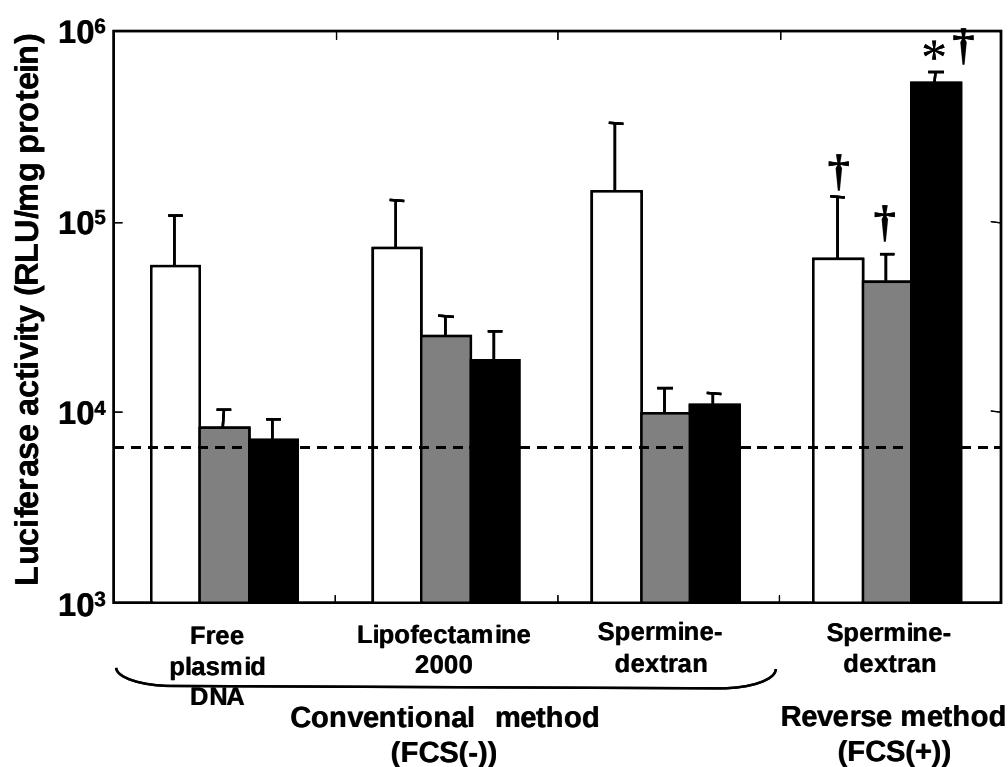
Figure 2. Time course of luciferase expression level for M \phi after transfection of luciferase plasmid DNA with the spermine-dextran by the conventional and reverse methods. The cells were cultured for 2 (open bars), 4 (light gray bars), and 6 (solid bars) days in the presence (FCS(+)) or absence of FCS (FCS(-)). The dotted line indicates the level of non-transfected, original M \phi . *, p < 0.05 ; versus the expression level of spermine-dextran-plasmid DNA complexes by the conventional method at the corresponding time. †, p < 0.05 ; versus the expression level of free plasmid DNA at the corresponding time.
