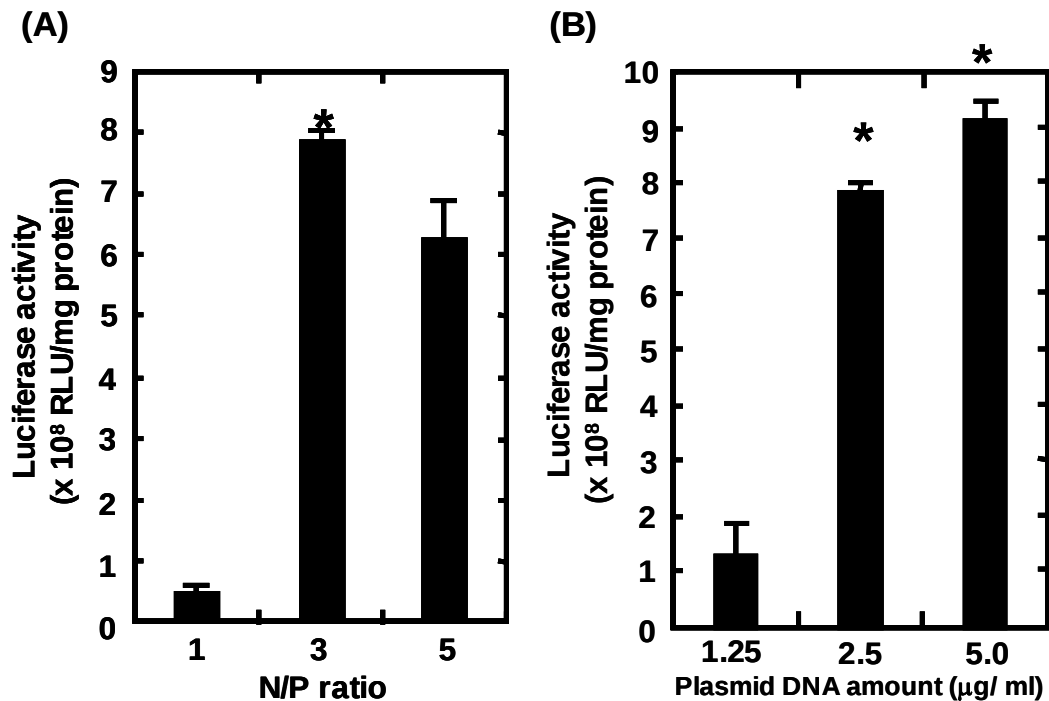
Figure 5. (A) Effect of the N/P ratio on the level of gene expression of spermine-pullulan-plasmid DNA complexes for HepG2 cells. The plasmid DNA amount is 5 \mu\text{g/well} . The molecular weight of pullulan used for spermine introduction is 47,300. *, p < 0.05 ; versus the expression level of complexes prepared at other N/P ratios. (B) Effect of the plasmid DNA amount on the level of gene expression of spermine-pullulan-plasmid DNA complexes for HepG2 cells. The N/P ratio is 3.0. The molecular weight of pullulan used for spermine introduction is 47,300. *, p < 0.05 ; versus the expression level of complexes at other plasmid DNA amounts.
