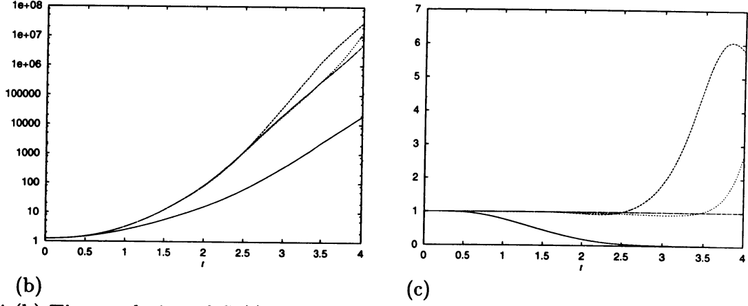
Fig.4 (b) Time evolution of S_n(t) for n = 0 (solid), 1 (dashed), 2 (short-dashed), 5 (dotted) and \infty (dash-dotted). (c) Time evolution of R_n(t) for n = 0 (solid), 1 (dashed), 2 (short-dashed), 5 (dotted) and 10 (dash-dotted).
