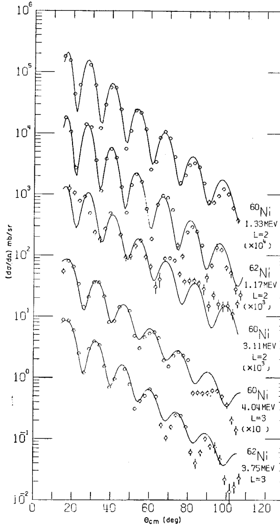
Fig. 6. The angular distributions covering a wide angular range obtained for the strongly excited states of ^{60}\text{Ni} and ^{62}\text{Ni} . The solid curves are the DWBA predictions.
