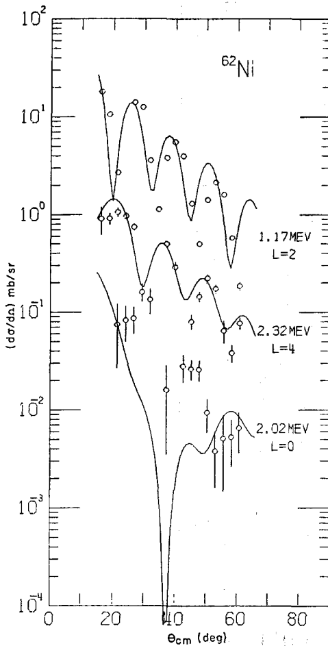
Fig. 8. Comparison of the measured angular distributions and the predictions of the DWBA calculation using the quasi-particle model form factors calculated by Glendenning and Veneroni.
