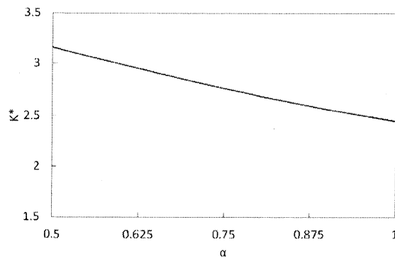
Figure 5: Comparative static effects of \alpha on optimal capital investment
