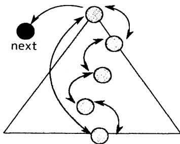
図 12: topdown-extract-min
