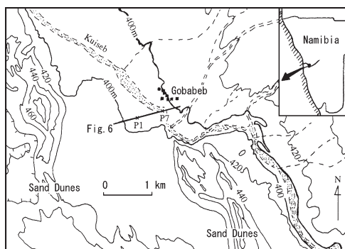
Fig. 1. Study area. P1, P7: Soil profile (Fig. 14).
