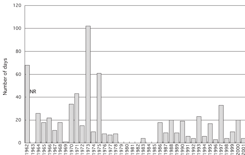
Fig. 16. Summary of Kuiseb River flooding at Gobabeb, 1962–2001.
