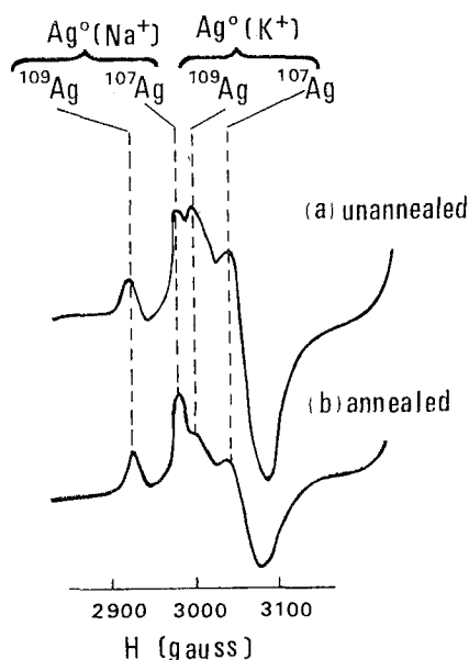
Fig. 9. Low-field parts of ESR spectra by Ag^{\circ} in 6.7 Na 2 O·13.3 K 2 O·80 SiO 2 glass (Imagawa 21) ).
