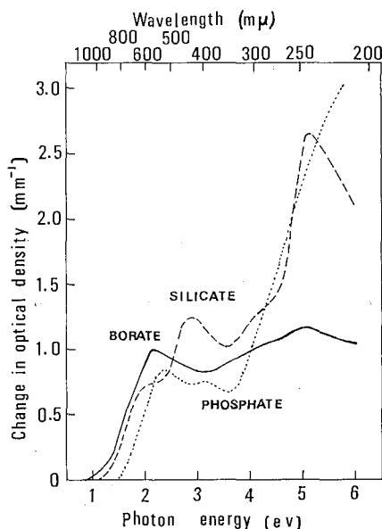
Fig. 1. Radiation-induced absorption in a silicate glass ( 2\text{SiO}_2 \cdot 0.35\text{Na}_2\text{O} \cdot 0.3\text{CaO} ), a borate glass ( \text{B}_2\text{O}_3 \cdot 0.35\text{Na}_2\text{O} \cdot 0.3\text{CaO} ) and a phosphate glass ( \text{P}_2\text{O}_5 \cdot 0.35\text{Na}_2\text{O} \cdot 0.3\text{CaO} ) (Bishay and Ferguson 3) ).
