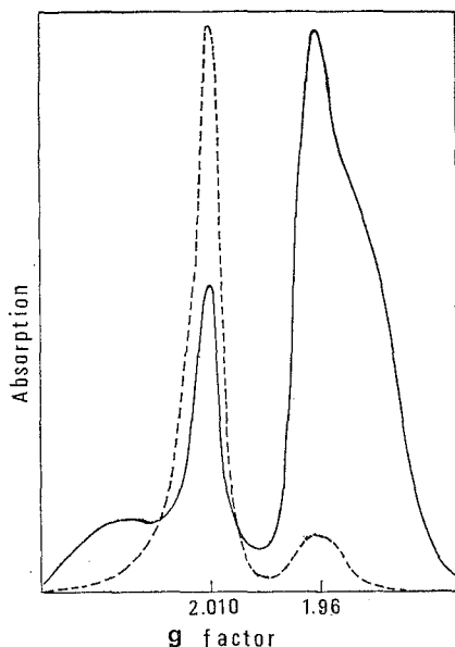
Fig. 6. ESR spectrum of \text{Na}_2\text{O} \cdot 3\text{SiO}_2 glass exposed to 10^5 r x-rays (Stroud, Schreurs and Tucker 9) ). --- No cerium added, — 35 \times 10^{18} \text{ Ce}^{3+}/\text{cm}^3 , 0.3 \times 10^{18} \text{ Ce}^{4+}/\text{cm}^3 . Divide the solid curve ordinates by 12.5.
