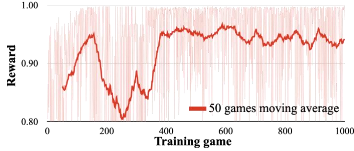
Fig. 5 Variation of moving average of reward during the training
