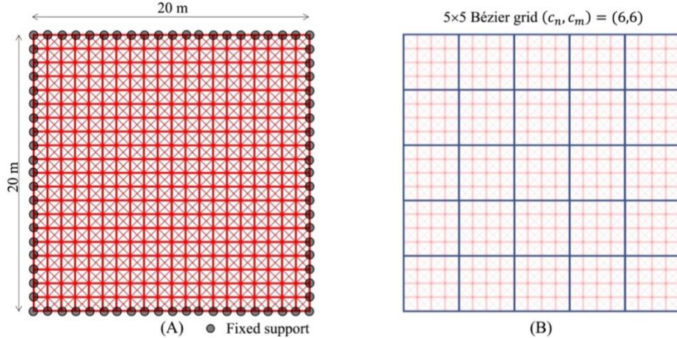
Fig. 10 20 \times 20 -grid latticed shell (fully braced) with (c_n, c_m) = (6,6) ; (A) Structural model 1, (B) Bézier control net
