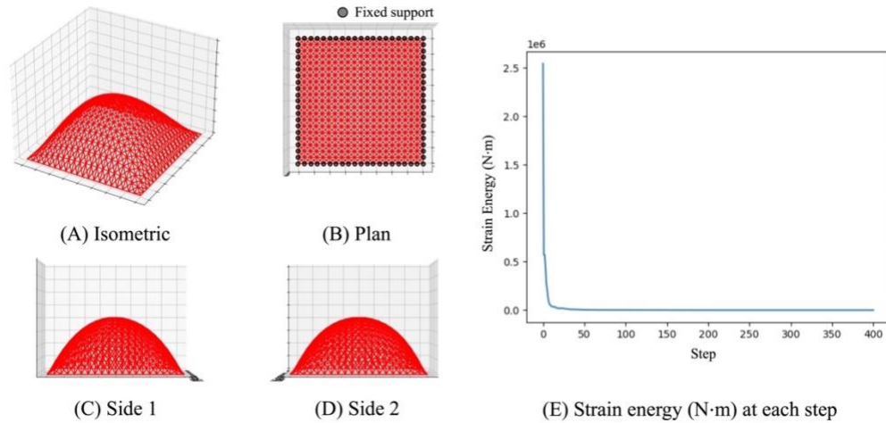
Fig. 11 20 \times 20 -grid shell: Structural model 1
