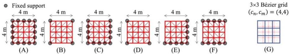
Fig. 4 Structural models 1–6 for the training phase with c_n = c_m = 4 for the Bernstein basis functions; (A) Model 1, (B) Model 2, (C) Model 3, (D) Model 4, (E) Model 5, (F) Model 6, (G) Bézier control net
