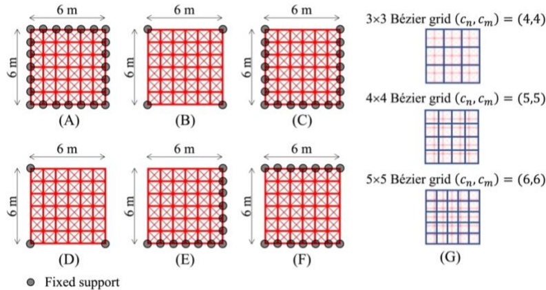
Fig. 6 6×6-grid latticed shells (fully braced) with (c_n, c_m) = (4,4) , (5,5) , and (6,6) ; (A) Model 1, (B) Model 2, (C) Model 3, (D) Model 4, (E) Model 5, (F) Model 6, (G) Bézier control nets
