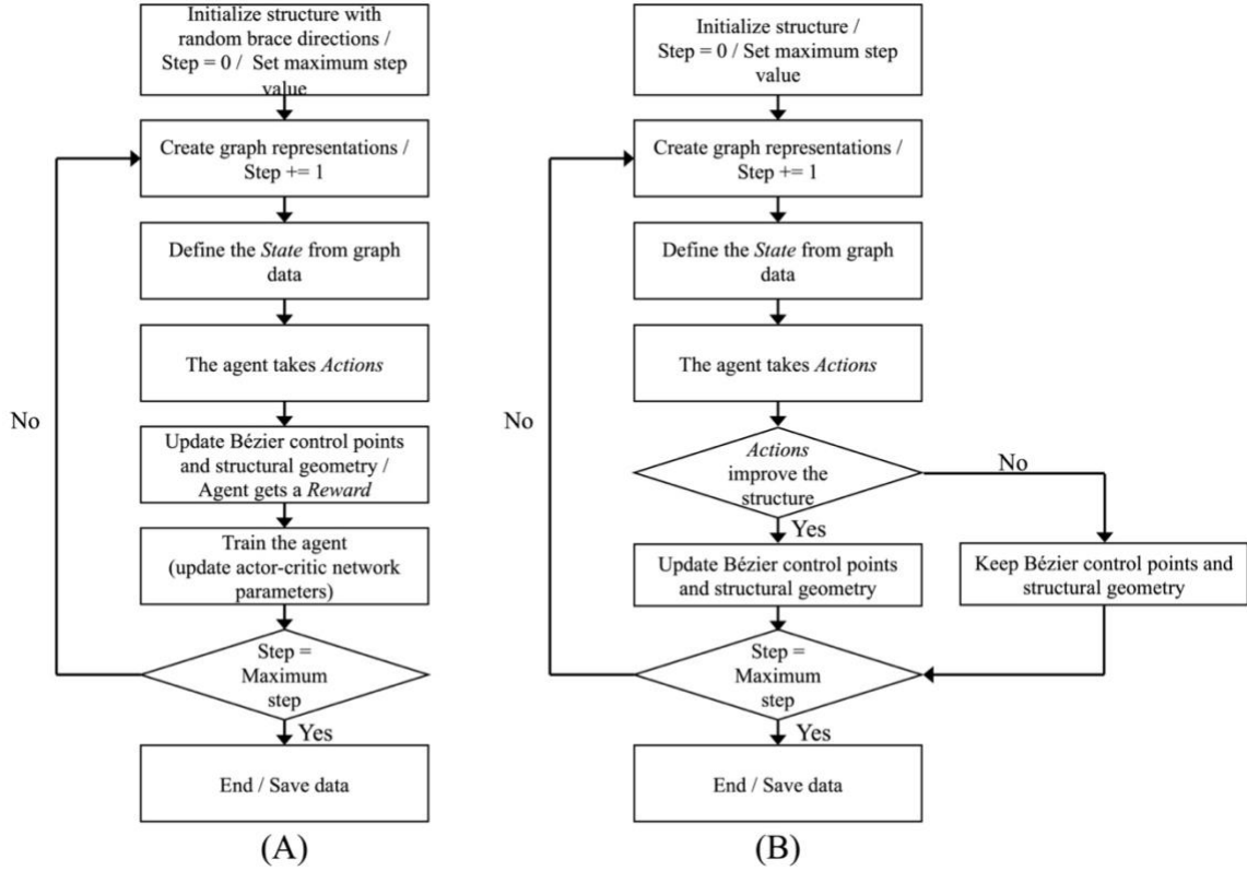
Fig. 3 The algorithms; (A) Training phase, (B) Test phase
