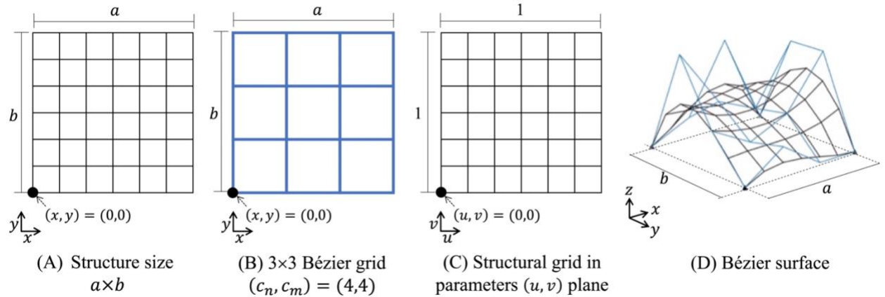
Fig. 1 Bézier surface of the latticed shell defined by Bézier control net.
