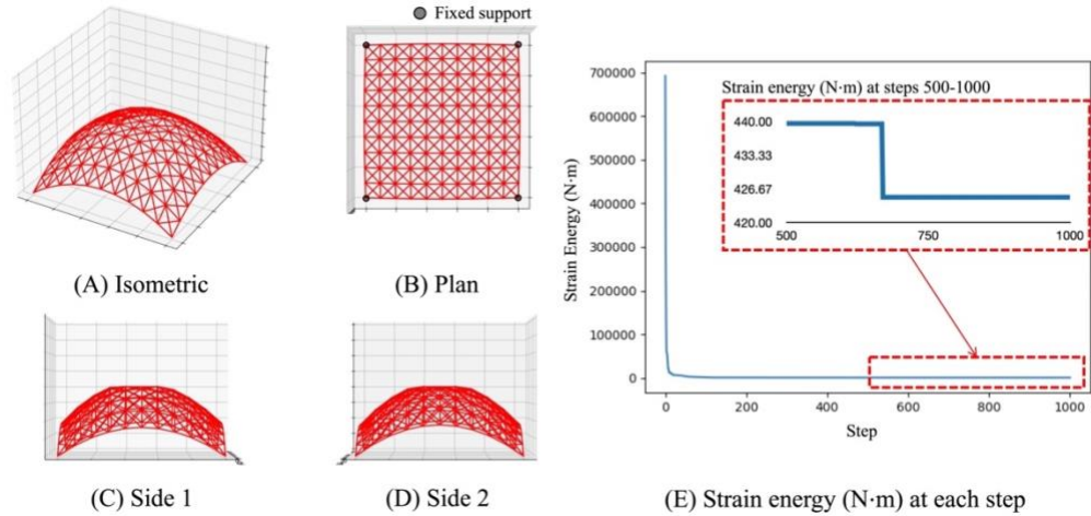
Fig. 9 10×10-grid shell: Structural model 2
