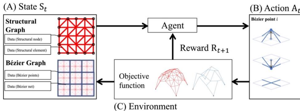
Fig. 2 Proposed MDP for geometry optimization of latticed shells with Bézier surface
