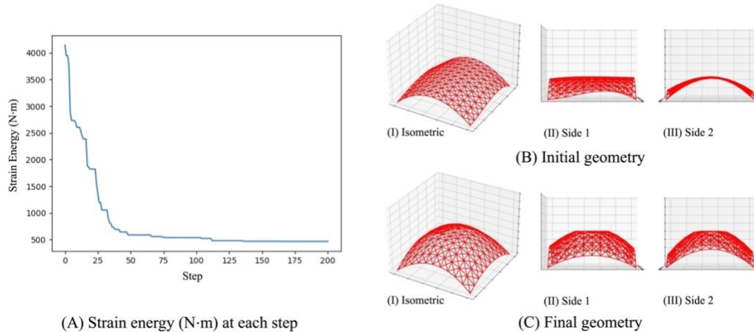
Fig. 13 10×10-grid latticed shell with initial irregular geometry: Structural model 2
