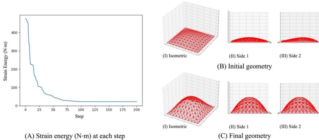
Fig. 12 10×10-grid latticed shell with initial irregular geometry: Structural model 1
