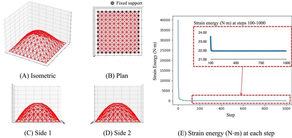
Fig. 8 10×10-grid shell: Structural model 1
