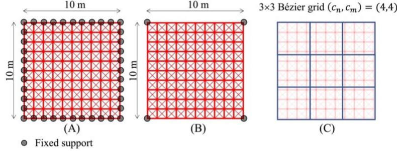
Fig. 7 10×10-grid latticed shells (fully braced) with (c_n, c_m) = (4,4) ; (A) Model 1, (B) Model 2, (C) Bézier control net
